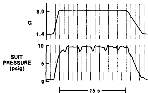
Fig. 8. Anti-G suit pressure during high-G training. Because the trainee's abdominal wall relaxes and the abdominal bladder of the suit expands during the inspiratory phase of the AGSM, the resulting pressure swings in the suit allow the trainer to monitor and record the rhythm, and to some extent the vigor, of the trainee's straining.
