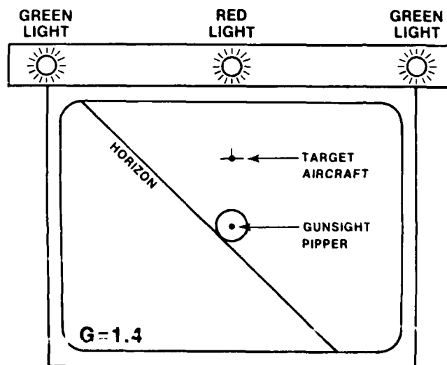
Fig. 6. Light bar and video display viewed by trainee during centrifuge runs. On the GOR he fixates the central red light of the light bar while monitoring the intensity of the peripheral green lights. During RORs (except the final one) he tracks the aircraft symbol to maintain the desired G level. Displayed horizon is veridical.
