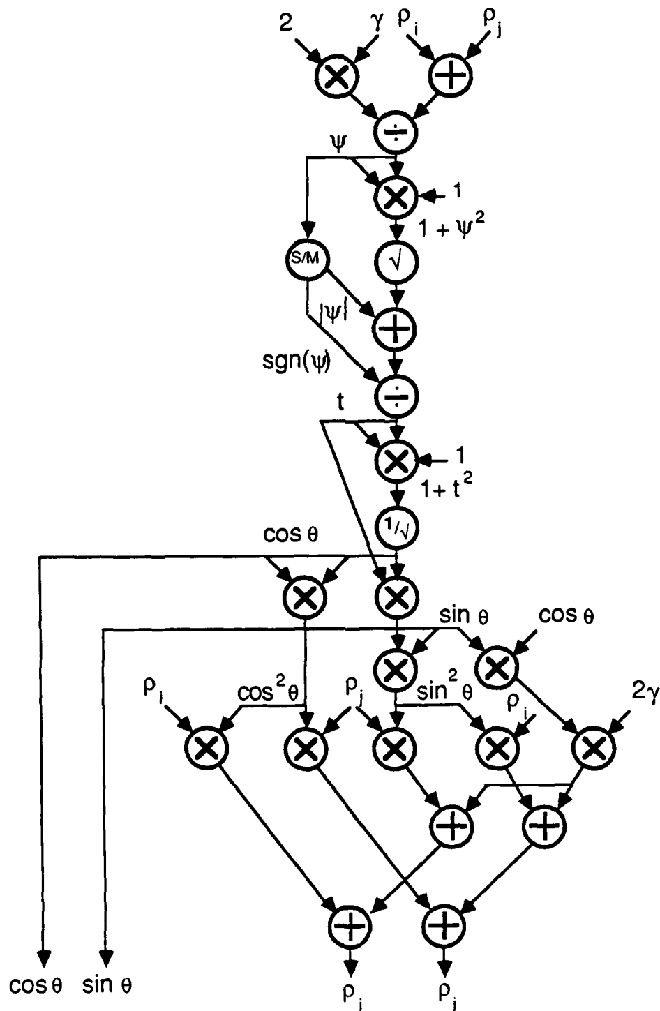
Figure 9.4.1.1: Dependency graph for the Rotation angle computation and Norm update in the Schimmel/Luk SVD architecture
