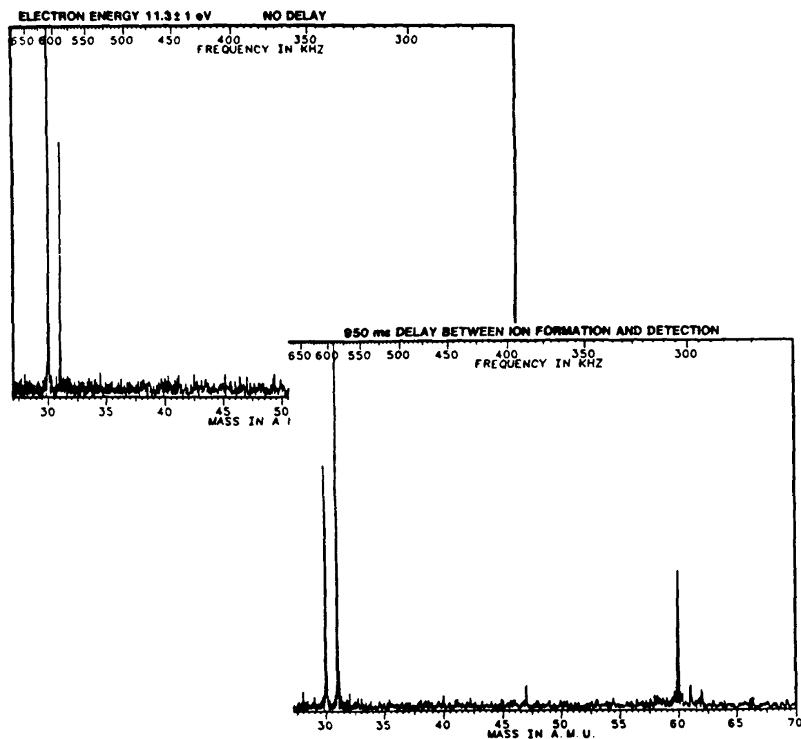
Figure 6.8: Evolution of \text{SiH}_3^+ and \text{SiH}_2^+ in 5% silane: argon. The nascent ion species distribution evolves rapidly to one dominated by \text{SiH}_3^+ and \text{Si}_2\text{H}_4^+ .
