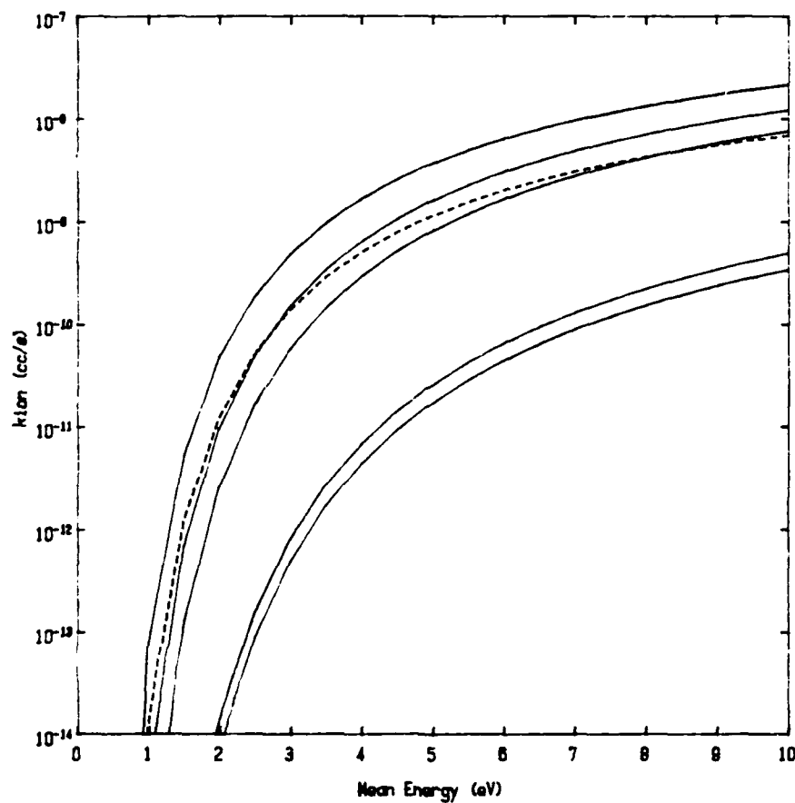
Figure 5.1: Ionization rates for maxwellian electron energy distributions in pure noble-gases (solid lines) and silane (dashed line). The x-axis is the mean electron energy of the \mathcal{F} basis function.
