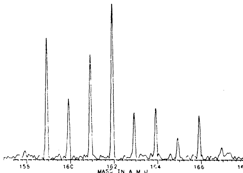
Figure 6.19: \text{Xe}^+ reaction with silane showing the production of condensation products \text{XeSiH}_n^+ for n = 2, 3 .
