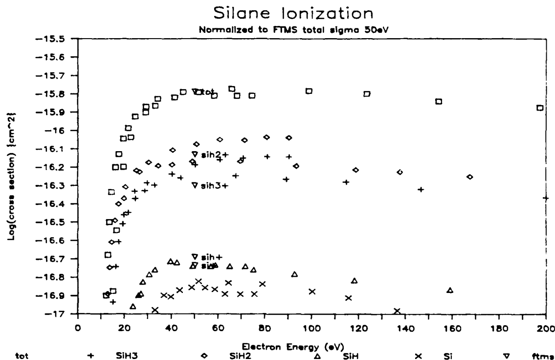
Figure 3.10: Partial ionization cross-sections of Chatham and Turban scaled by the present total cross-section observed at 50 eV.
