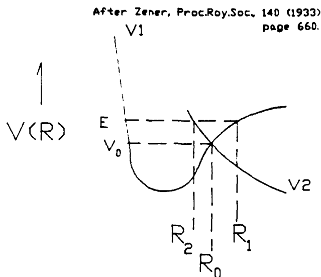
Figure 7.4: Potential energy surfaces and reference points for the tunneling calculation after the treatment of Zener (see text).
