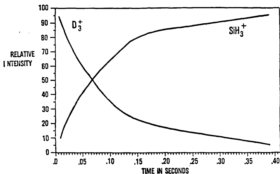
Figure 6.11: Reaction of D_3^+ with silane. The absence of deuterated silicon hydride cations in the product mass spectrum demonstrates hydride transfer is preferred to elimination of H_2 from an ion complex.
