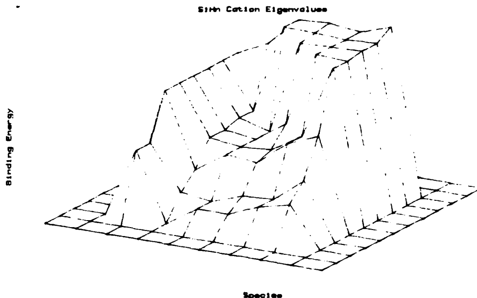
Figure 7.2: UHF eigenvalue spectra for the silicon hydride cations using geometries optimized at the MP2/6-31g** level. Vertices correspond to one electron binding energies. The flat base is at an energy of -30\text{eV} . From left to right the ridges correspond to \text{SiH}_4 , \text{SiH}_n^+ n = 4, 3, 2, 1, 0 . Recall that the \text{SiH}_4 t_2 and a_1 orbitals are at -13.1 and -19.9\text{eV} , respectively. Highest occupied molecular orbitals, indicated by circles, of \text{SiH}_n for n=4, 3 , and 2 are lower in energy than those for n=0, 1 .
