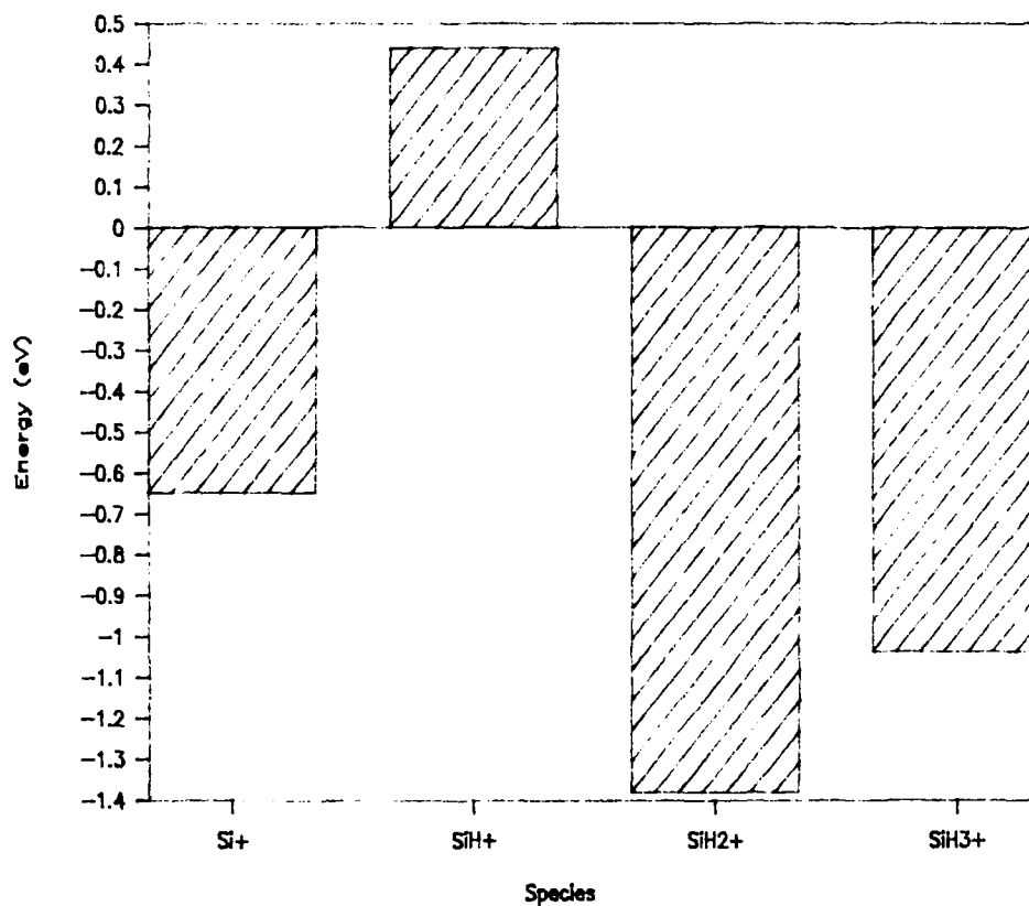
Figure 3.5: MP4/6-31g** enthalpies for the silicon hydride cations at their MP2/6-31g** geometries compared to those of the T_d cation whose geometry is identical to that of neutral silane. Zero-point energy corrections for the ions and hydrogen molecules are from MP2 frequency calculations for the silicon hydride species and exact values for H_2 .
