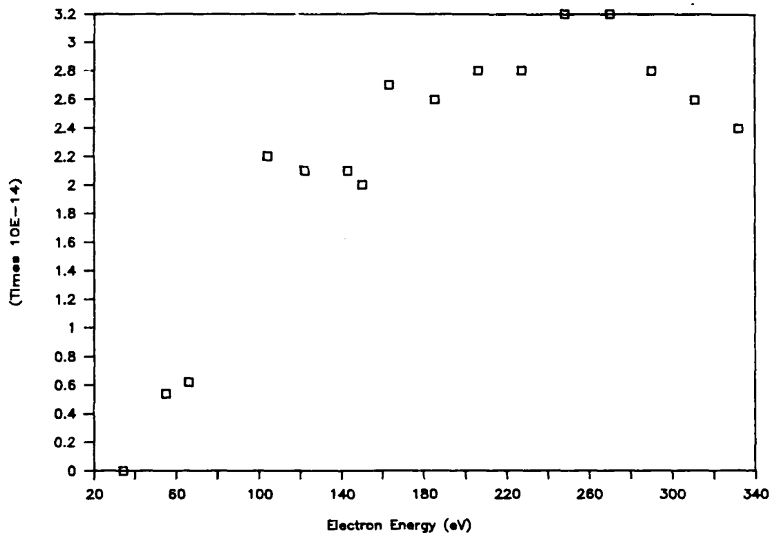
Figure 2.16: \sigma_{12}(\text{Ne}) inferred from the ratio of \text{Ne}^{2+} to \text{Ne}^+ ICR signals at 150 millisecond irradiation times with various energies. Uncertainty is \approx \pm 10^{-14} \text{ cm}^2 .
