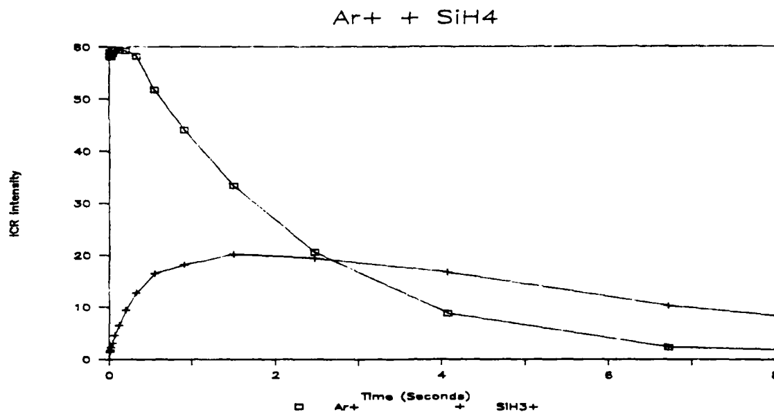
Figure 6.16: \text{Ar}^+ reaction with silane as observed by FTMS. The product \text{SiH}_3^+ reacts only slowly with silane to yield \text{Si}_2\text{H}_5^+ (not shown).
