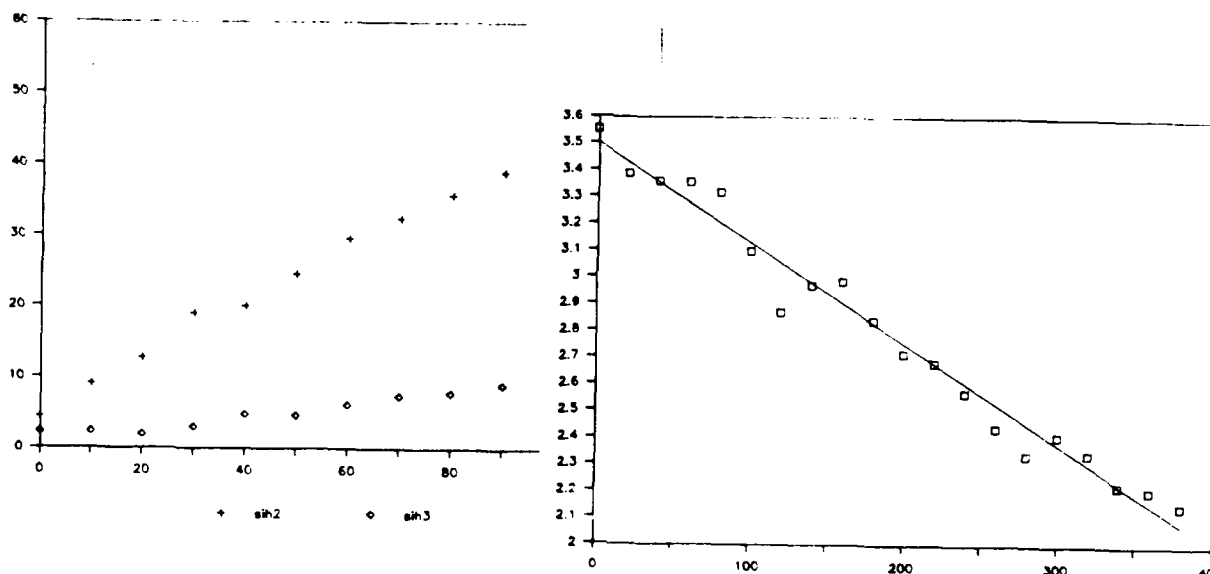
Figure 6.18: Xe^+ reaction with silane showing the evolution of SiH_n^+ for n = 2, 3 . Most, if not all, of the trihydride may be accounted for by the rapid hydride transfer from silane to SiH_2^+ .
