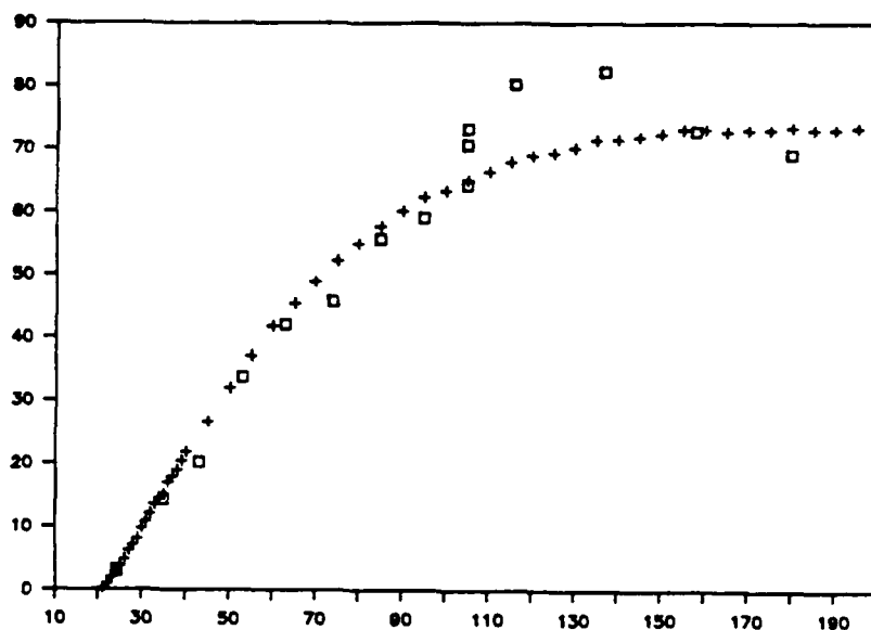
Figure 2.12: Ionization cross section, \sigma_1 , from the ratio of FTMS signal to electron beam current (squares) scaled to the absolute values from the crossed-beam experiments of Wetzel at 50 eV.
