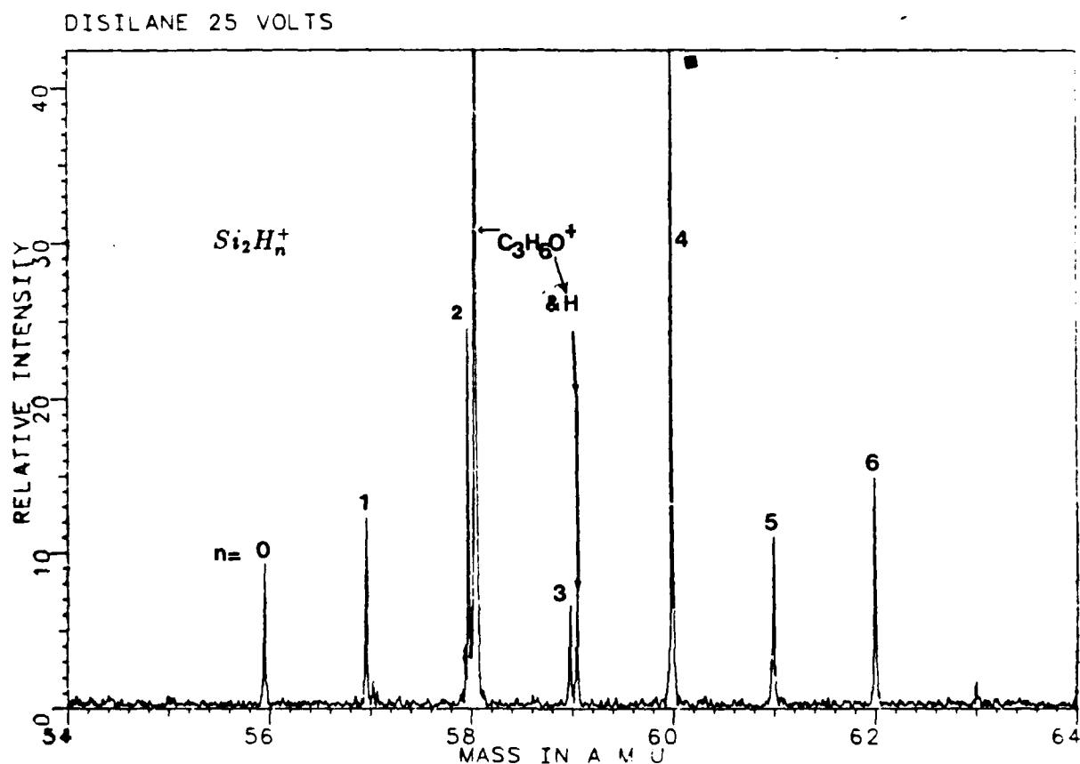
Figure 6.9: 25 eV electron impact mass spectrum of disilane. The right-hand isotopic peaks at m/e 58 and 59 are from background acetone in the vacuum system. The relative peak intensities are roughly independent of electron energy above 20 volts.
