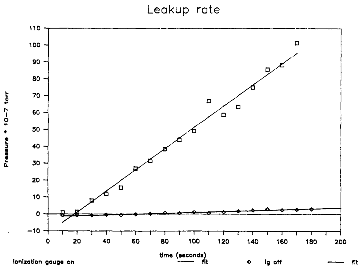
Figure 2.7: Vacuum chamber leak rate with and without the nude ionization gauge turned on as measured with the spinning rotor friction gauge. The hot nude gauge acts as a source of gas.
