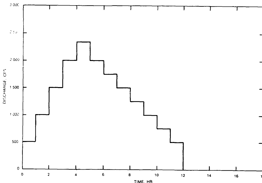
Figure 3. Synthetic hydrograph for scour comparison, Muddy Creek which scoured the channel invert on both sides of the downstream channel as shown in Photo 5. This design was deemed unsatisfactory.
