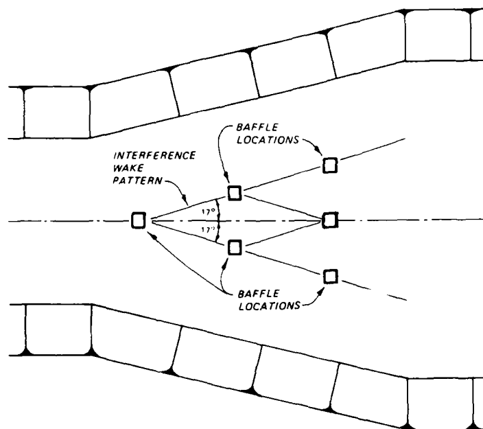
a. Baffle locations for maximum interference
