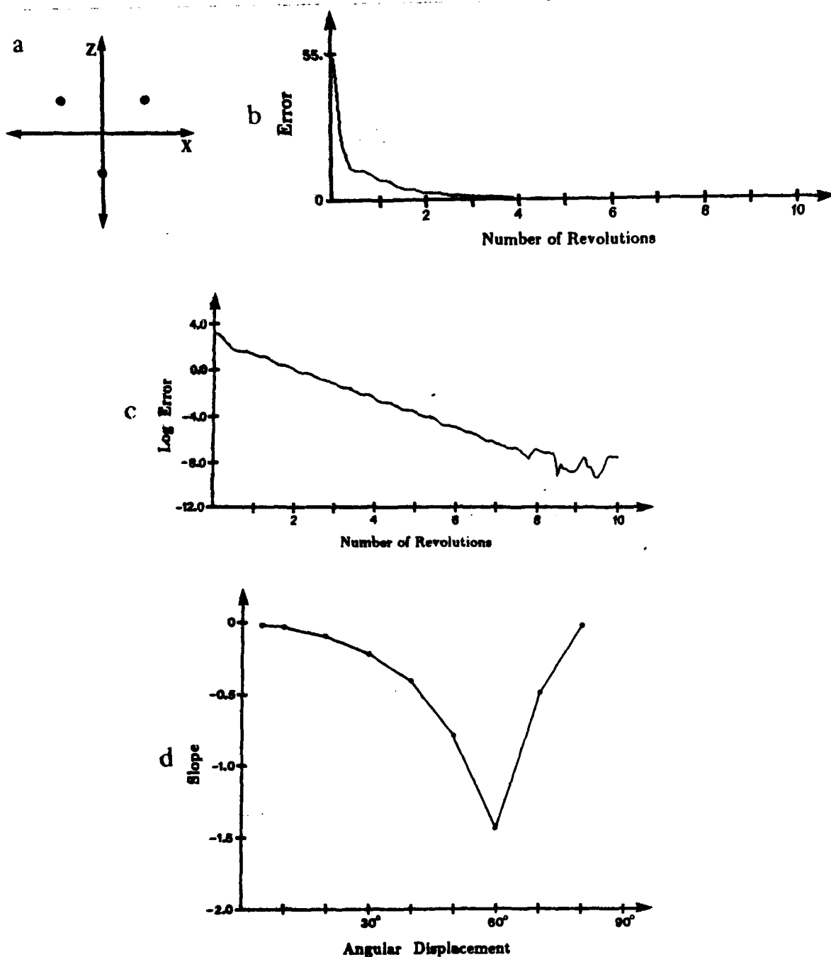
Figure 9. The results of computer simulations. (a) The true three point configuration, projected onto the X-Z plane. (b) The error in the computed 3-D model, as a function of time, for 20 displacements between frames. (c) The error in the 3-D model, plotted on a log scale. (d) The rate of convergence of the solution, as a function of the angular displacement between frames.
