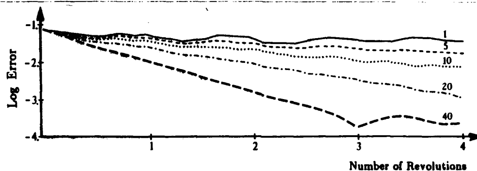
Figure 4. Graphs of the error in the internal distances between points in the computed 3 D model, as a function of time, plotted on a log scale. The points are rotated 4 full revolutions, in steps of 40^\circ , 20^\circ , 10^\circ , 5^\circ and 1^\circ . The graphs are shown superimposed, with the angular displacements indicated above each graph.
