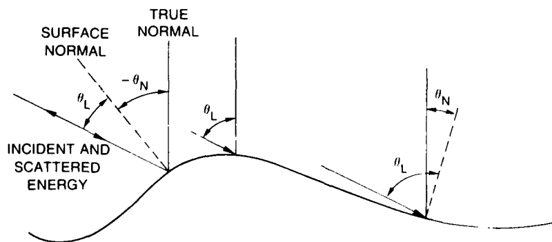
Fig. A3 — Local incidence angle of the radar signal is determined by the depression angle at the radar and the local slope of the long wave at the point of incidence and causes tilt modulation of the expression of Eq. (3)
