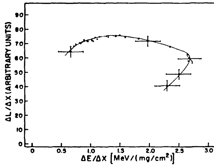
Figure 1-10 Specific luminescence as a function of specific energy loss for 4 He ions transiting 112 \mu\text{g}/\text{cm}^2 NE 102 scintillator. Taken from Ref. [18].
