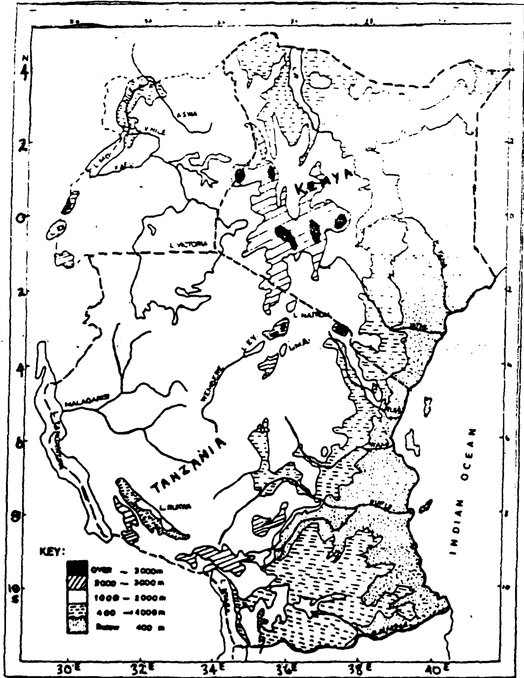
Figure 1.1.1. Physical Features of East Africa (From Nyenzi, 1979).
