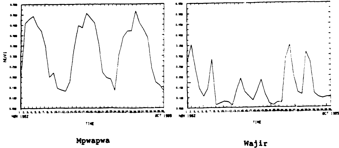
Figure 3.1.3 b Comparison of NDVI time series from November 1982 to October 1985 at two stations.
