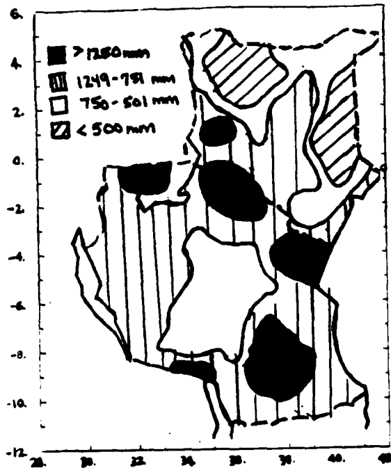
Figure 1.1.2. Average annual rainfall in East Africa
