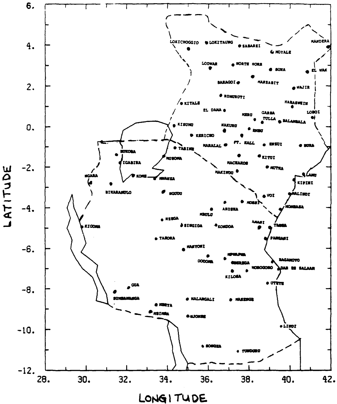
Figure 2.1. Location of stations used in this study.
