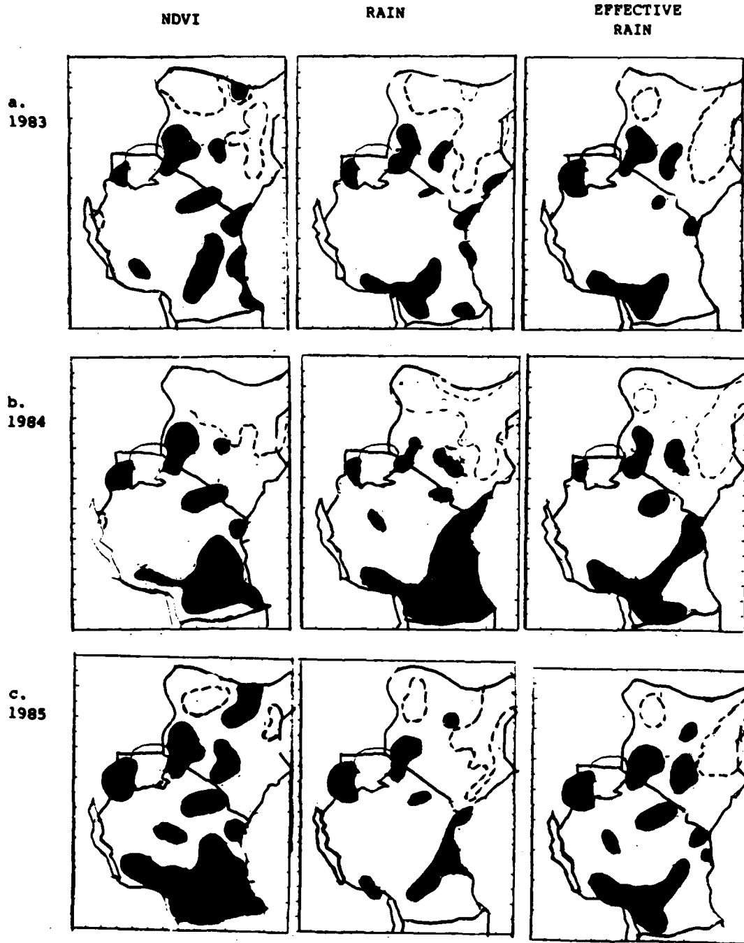
Figure 3.2.1. Annually-integrated NDVI, rainfall and effective rainfall for East Africa. Shaded areas indicate maximum values (NDVI > 4.0 , rain > 1000\text{mm} , effective rain > 0\text{mm} ), dashed lines enclose areas of minimum values (NDVI < 2.0 , rain < 500\text{mm} , effective rain < -1500\text{mm} ).
