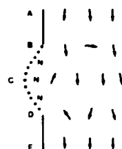
Figure 4. Diagrammatic representation of mean current directions at White Castle, Port Sulphur, and Natchez (Areas without current are marked with an "N." River stages were recorded at Donaldsonville, Louisiana)
