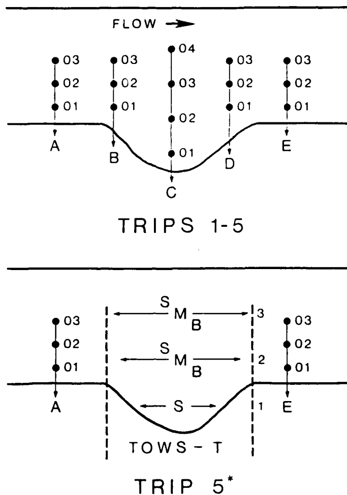
Figure 2. Diagram of station and transect configurations (larval fishes, zooplankton, and invertebrates were collected by towing in the eddy: S = surface, M = mid-depth, B = bottom)
