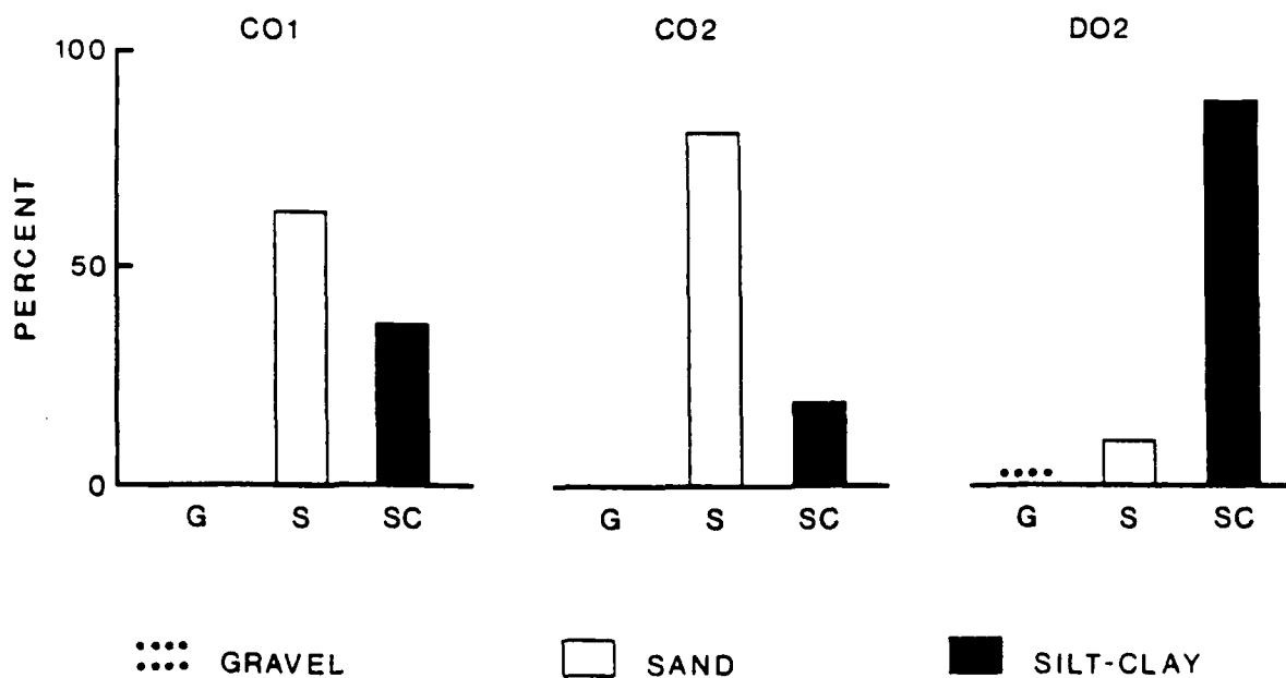
Figure B2. Sediment composition at stations near White Castle (Trips 3 and 5), 7 June and 19 July, 1985
