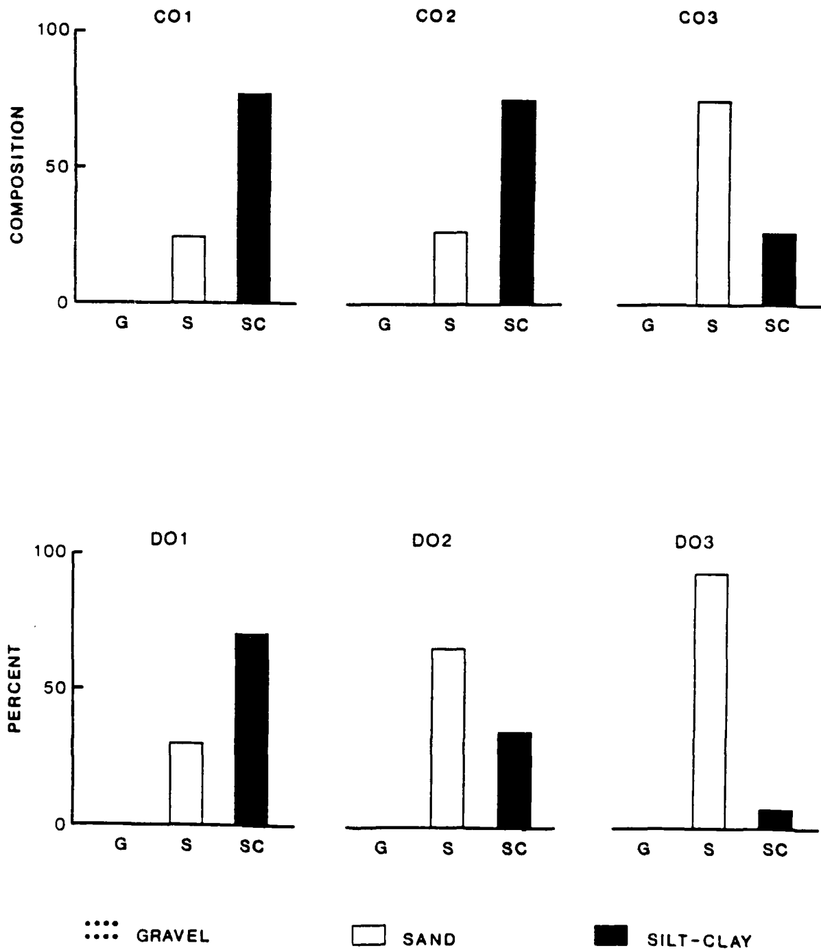
Figure B3. (Concluded)
