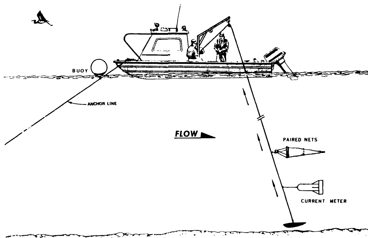
Figure 3. Schematic representation of sampling techniques
