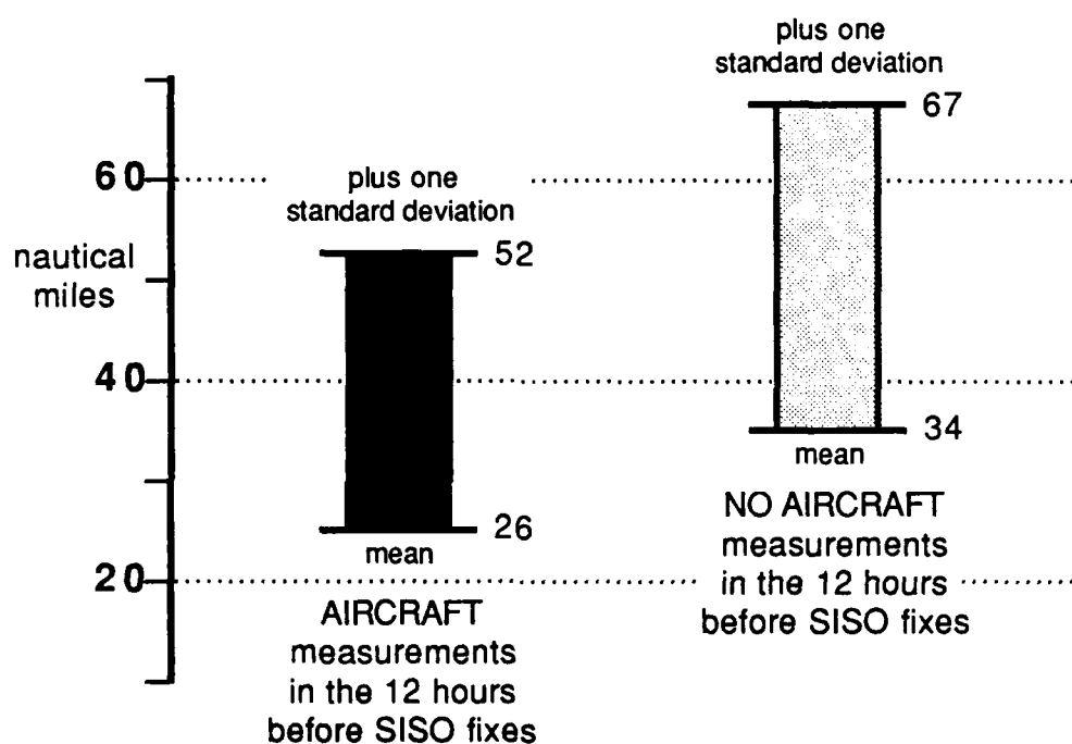
Figure 3.1: Comparison of mean and one standard deviation of fix position difference from Simultaneous Independent Satellite Observations (SISO). Diagram on the left shows fix difference when reconnaissance aircraft were present within 12 hours prior to the satellite fix times; diagram on the right gives information when no aircraft were available within 12 hours of fix time.
