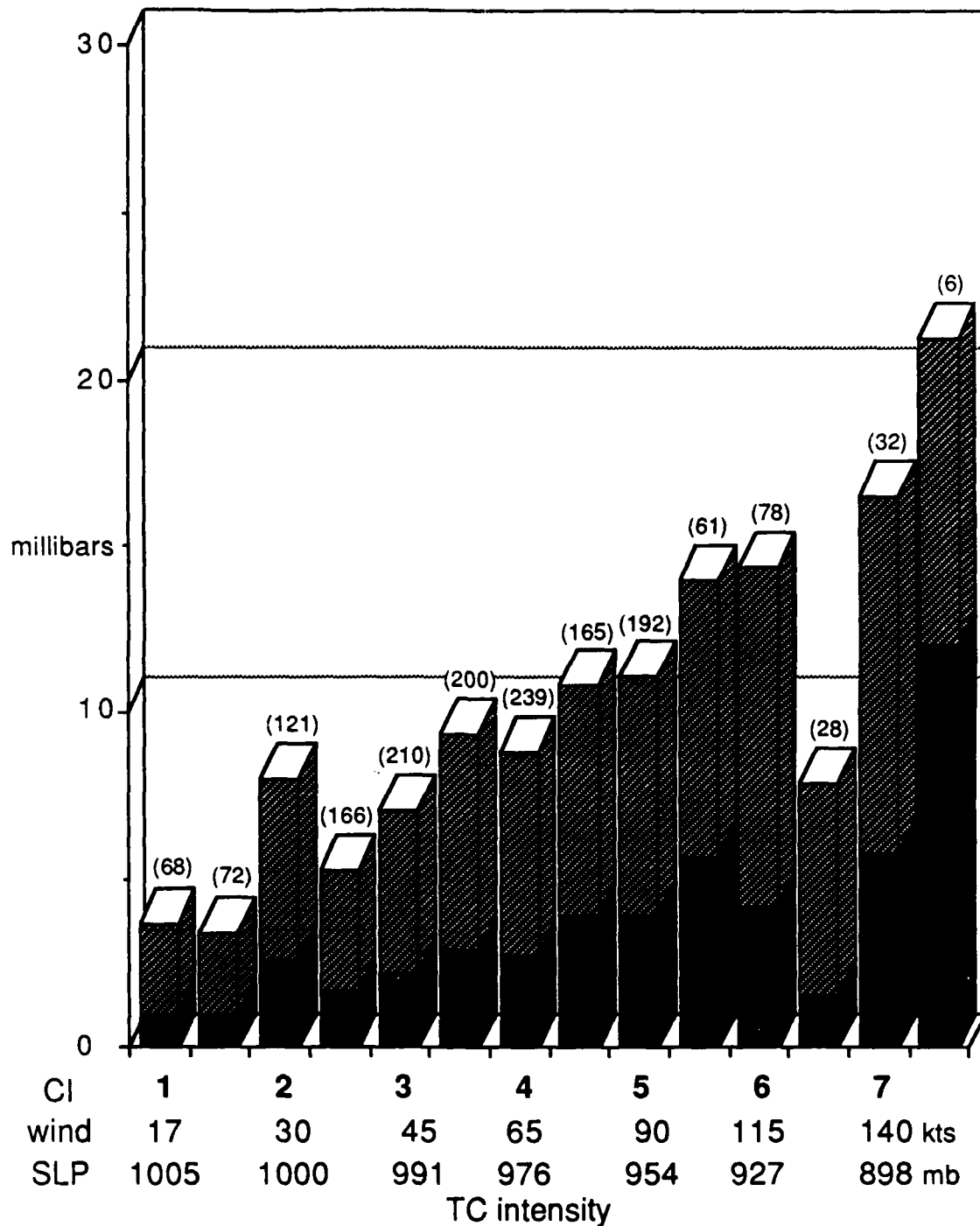
Figure 6.6: Intensity differences as a function of cyclone intensity, as measured by Simultaneous Independent Satellite Observations (SISO) observations. Mean (black) and one standard deviation (stippled shading) are indicated. Parentheses show number of cases.
