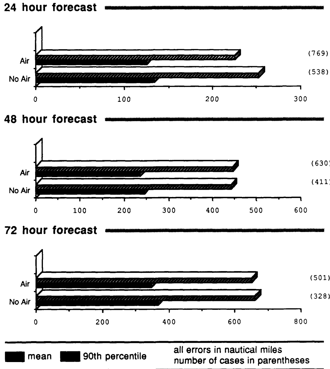
Figure 8.3: Same as Fig. 8.2 except for JTWC forecast of initially weaker intensity cyclones ( V_{max} \leq 45 kts).
