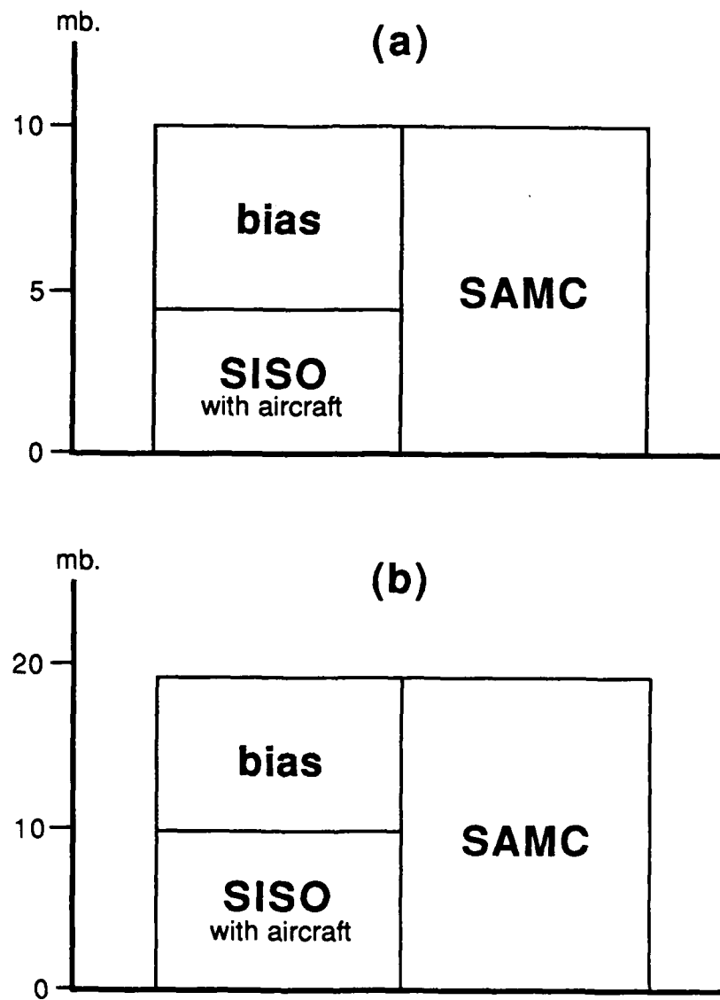
Figure 6.4: Comparison of mean (a) and mean plus one standard deviation (b) of SAMC and SISO that had prior aircraft intensity estimate differences. Shaded area shows the degree of SISO intensity bias.
