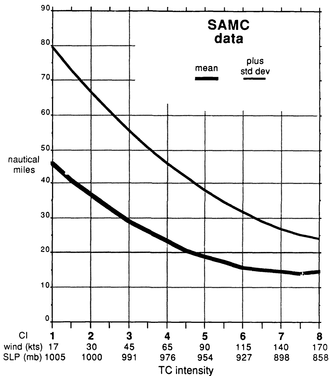
Figure 4.3: Mean plus one standard deviation of Satellite and Aircraft Measurement Comparison (SAMC) TC positioning differences as a function of cyclone intensity.
