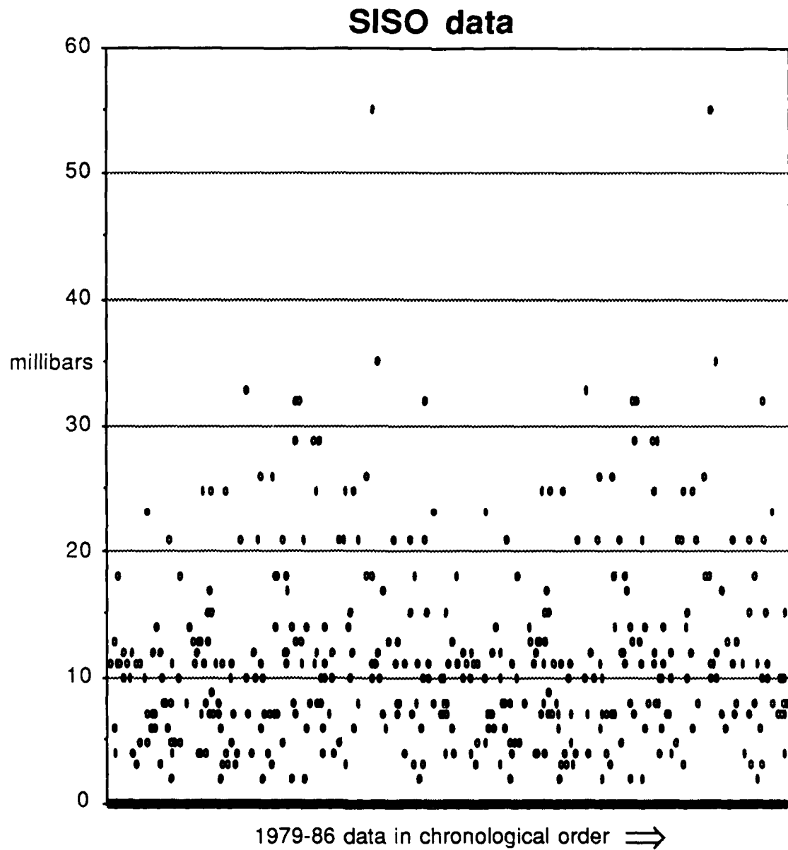
Figure 6.2: Simultaneous Independent Satellite Observations (SISO) of absolute TC Minimum Sea-Level Pressure intensity differences. Data clustering causes the thick black line at the 0 difference value.
