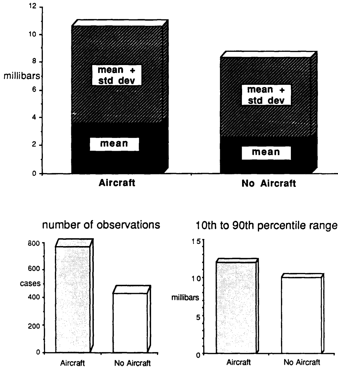
Figure 6.3: Comparison of Simultaneous Independent Satellite Observation (SISO) TC intensity differences between cases when aircraft measurements were and were not available in the 12 hours prior to the SISO measurement. Mean and one standard deviation values shown (top) along with the number of cases studied (lower left) and the range in values from the 10th to 90th percentiles (lower right).
