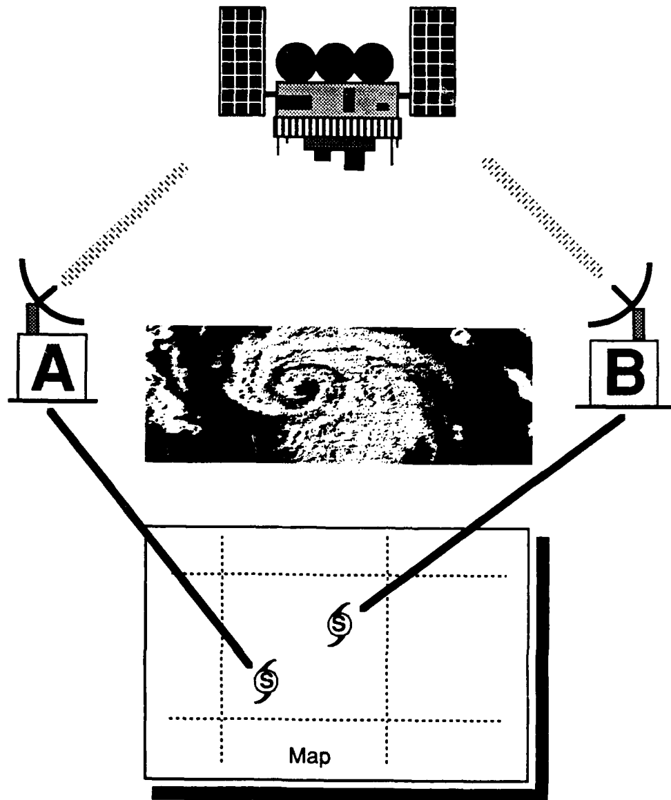
Figure 2.3: An illustration of Simultaneous Independent Satellite Observations (SISO). A satellite observes the tropical cyclone and two sites (A and B) receive and process the imagery information, simultaneously. This illustrates how simultaneous independent satellite fixes do not necessarily coincide with each other.
