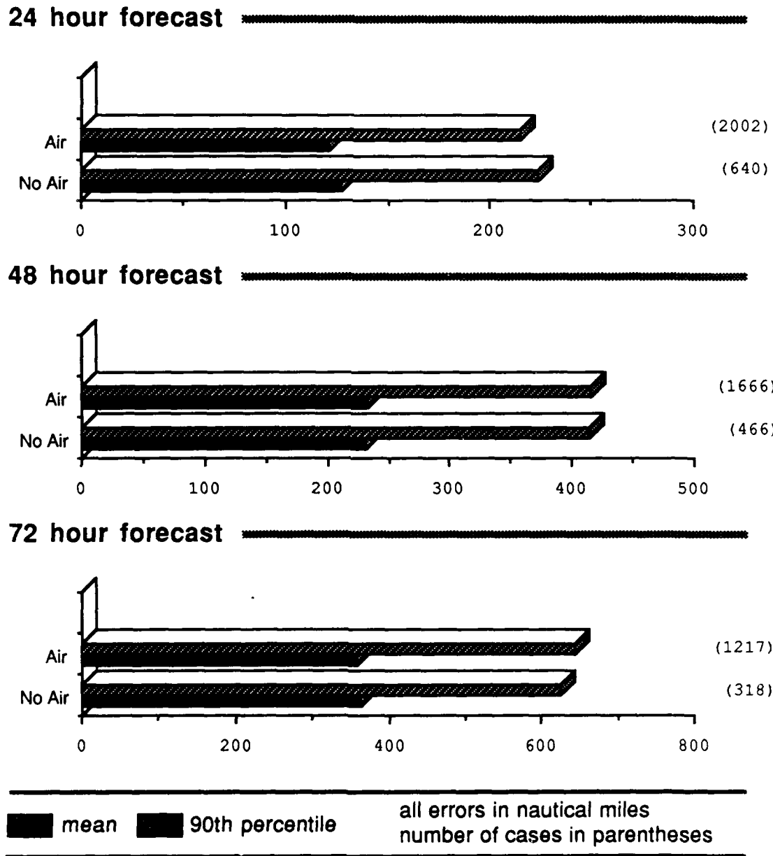
Figure 8.5: Same as Fig. 8.2 except for One-Way Tropical Cyclone Model (OTCM) forecasts.
