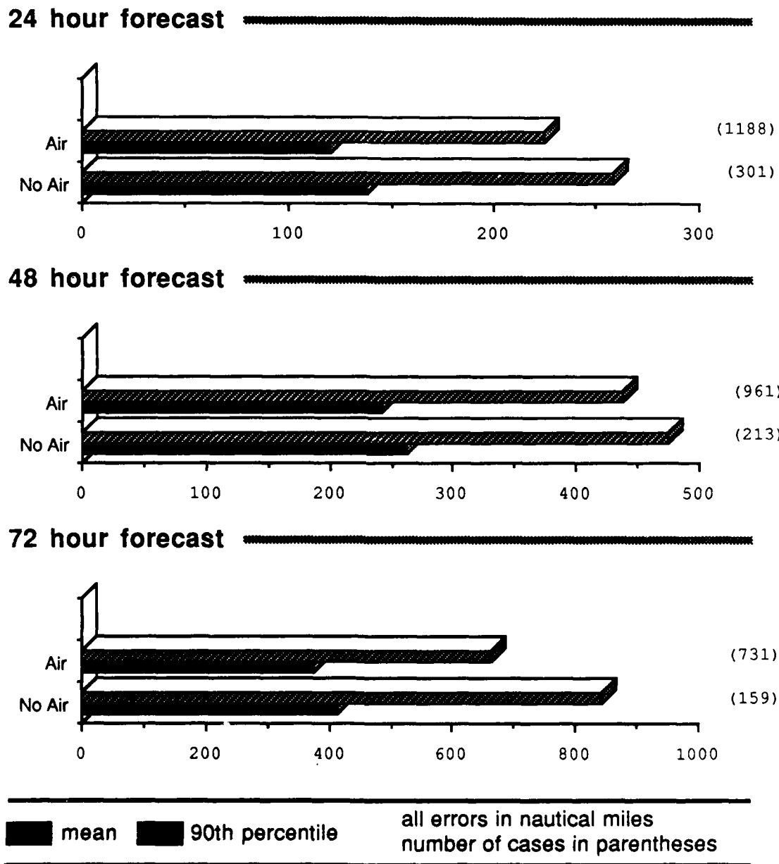
Figure 8.4: Same as Fig. 8.2 except for JTWC forecast of recurving cyclones ( V_{max} \leq 45 kts).
