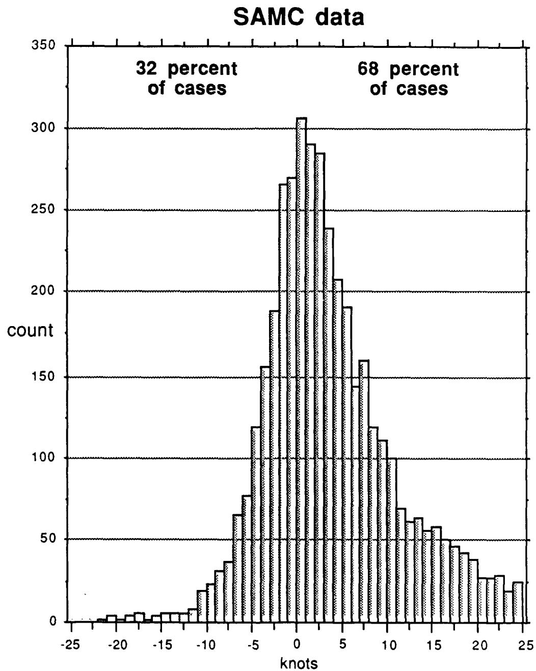
Figure 5.1: Frequency distribution of satellite minus aircraft TC speed differences from two consecutive satellite fixes minus two corresponding time-interpolated aircraft fixes. Information from the SAMC data set.
