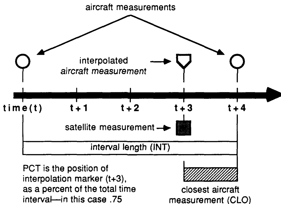
Figure 2.4: Illustration of the method of time interpolating of aircraft track position and intensity to satellite position times for fix and intensity comparisons. Aircraft measurements were made at times t and t+4 . Aircraft fix data were interpolated to the satellite fix time at t+3 . The total interval length from t to t+4 is recorded in the data set along with the time interval from the interpolated point at t+3 , the closest aircraft measurement at t+4 . The position of the interpolation is recorded as a percentage (PCT) of the total interval length.
