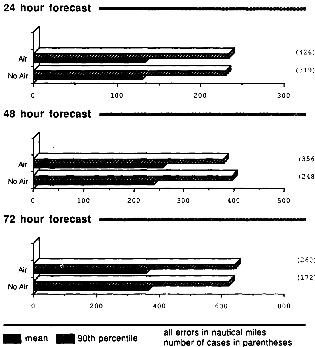
Figure 8.6: Same as Fig. 8.2 except for OTCM forecast of initially weaker intensity cyclones ( V_{max} \leq 45 kts).
