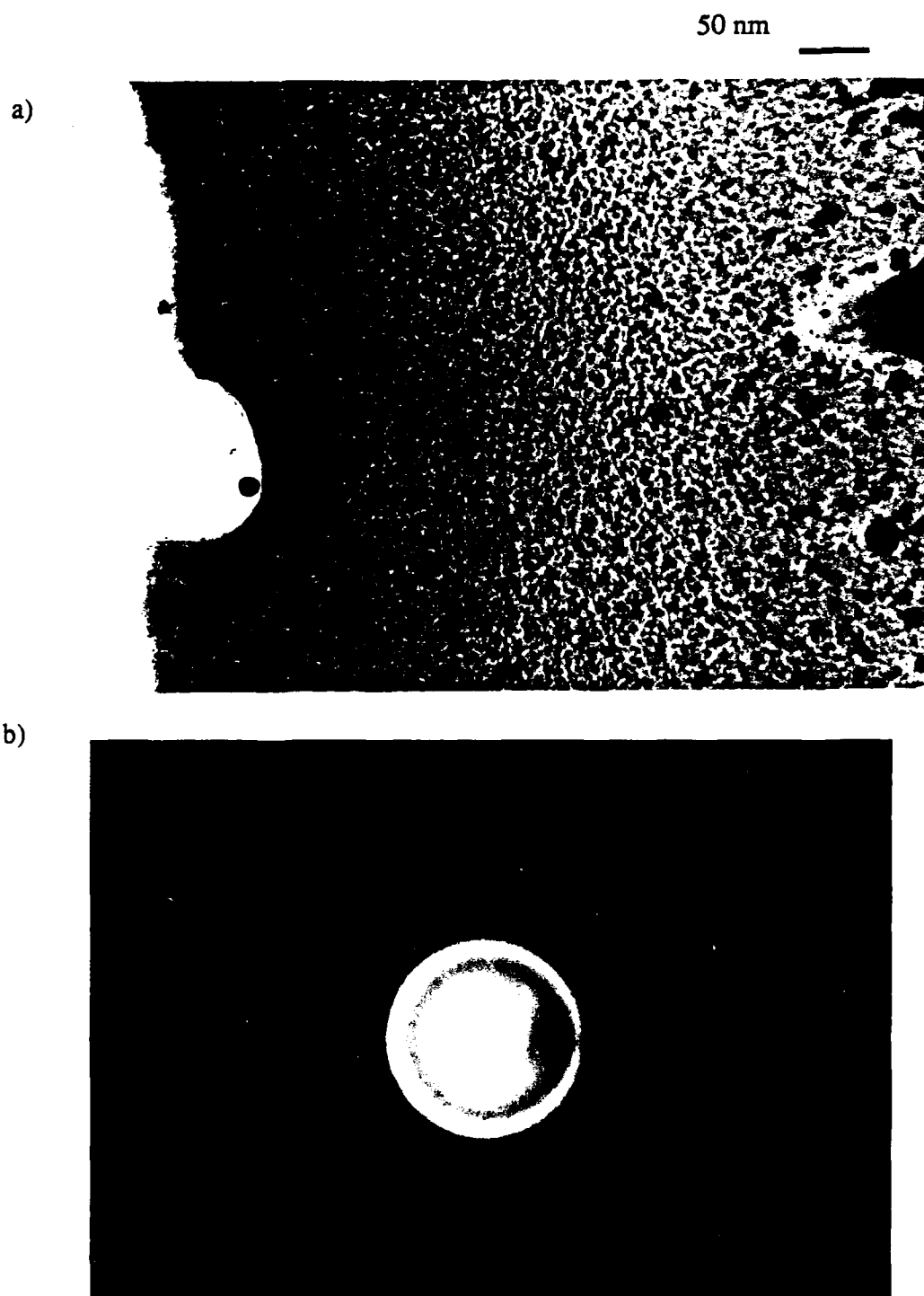
Figure 28 High Magnification TEM Micrograph a) Light underside region of Figure 27. Phase separated, modulated structure. b) Corresponding SAD
