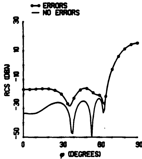
c. Bistatic scattering pattern, \phi_o = 90^\circ
