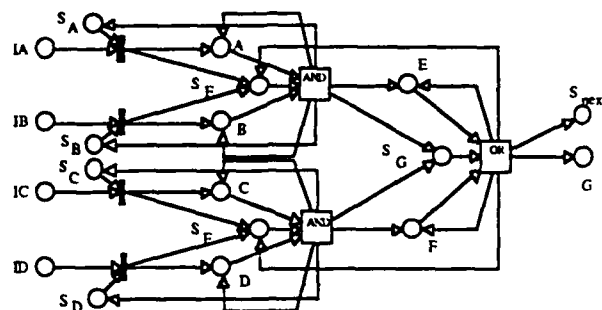
Figure 7 Inference net of a simple symbolic system, using the Predicate Transition Nets formalism
