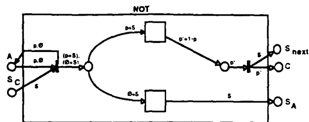
Figure 5 Model of the operator NOT
