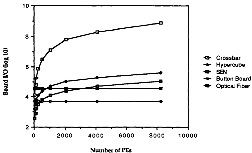
Figure 11. Board-level I/O as a function of the number of PEs/boards for B=10, M=2
