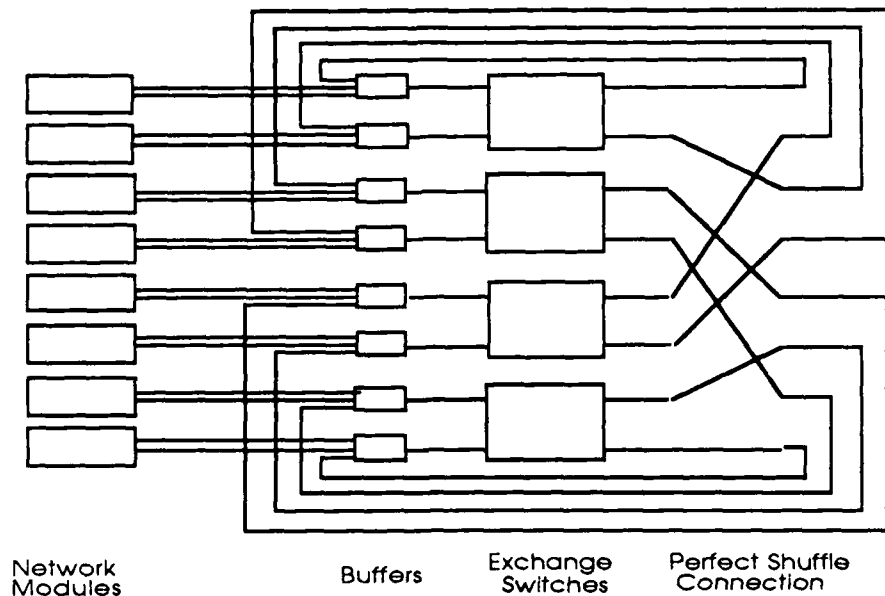
Figure 3. SEN for 8 PEs
