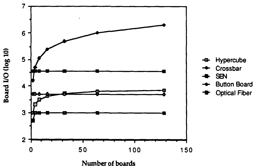
Figure 10. Board-level I/O as a function of the number of boards for B=32, N=16
