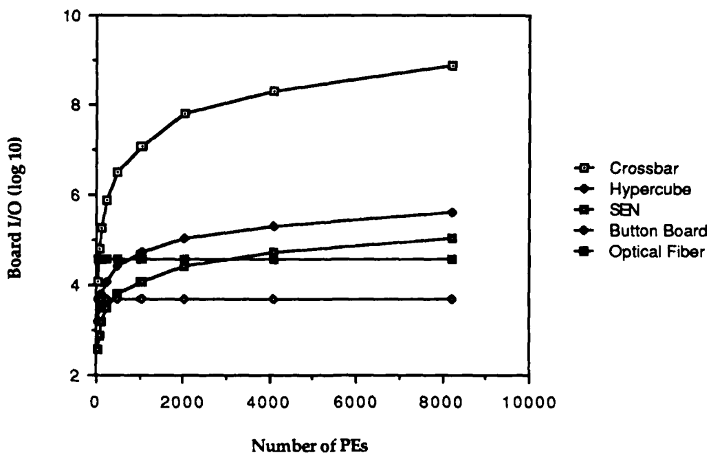
Figure 12. Board-level I/O as a function of the number of PEs/boards for B=100, M=16
