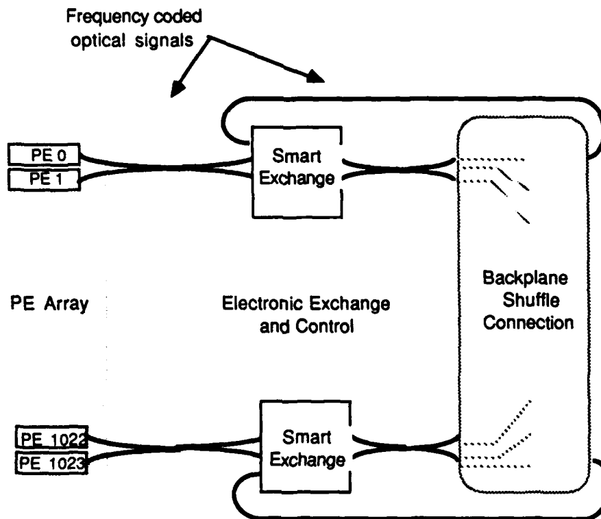
Figure 9. Serial electronic exchange parallel optical shuffle scheme
