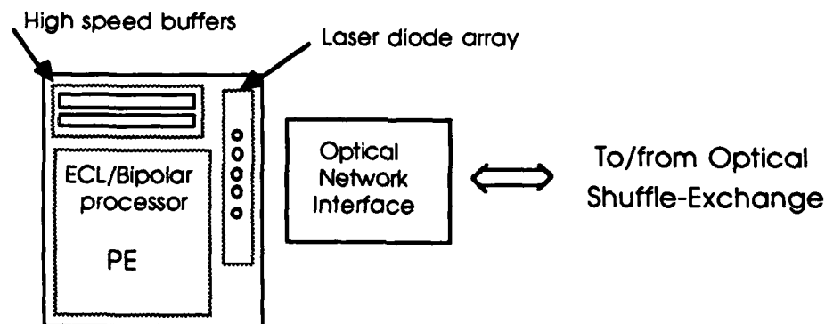
Figure 8. PE and optical SEN connection
