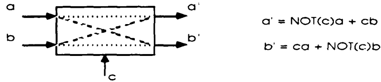
Figure 4. Basic Exchange Switch
