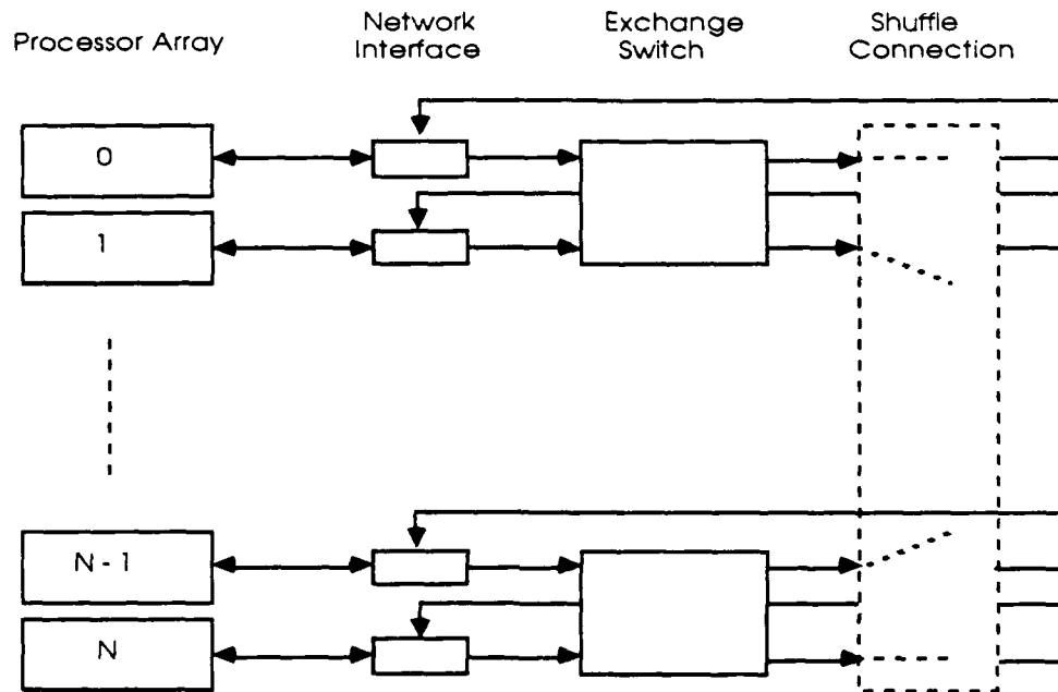
Figure 1. SEN and Processor Array Interface
