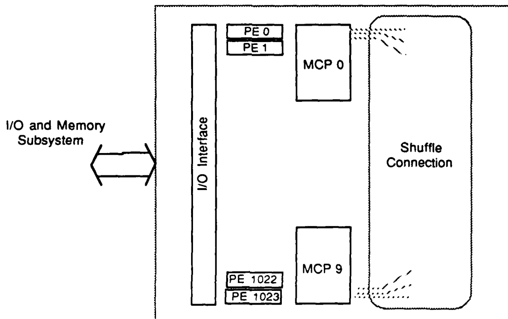
Figure 7. Scheme for an electronic SEN and PE array
