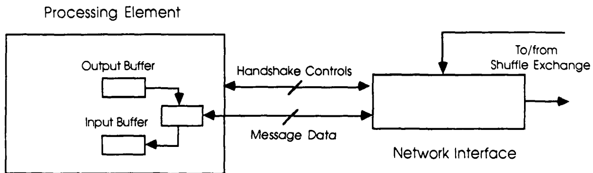
Figure 2. PE and Message Buffer interface
