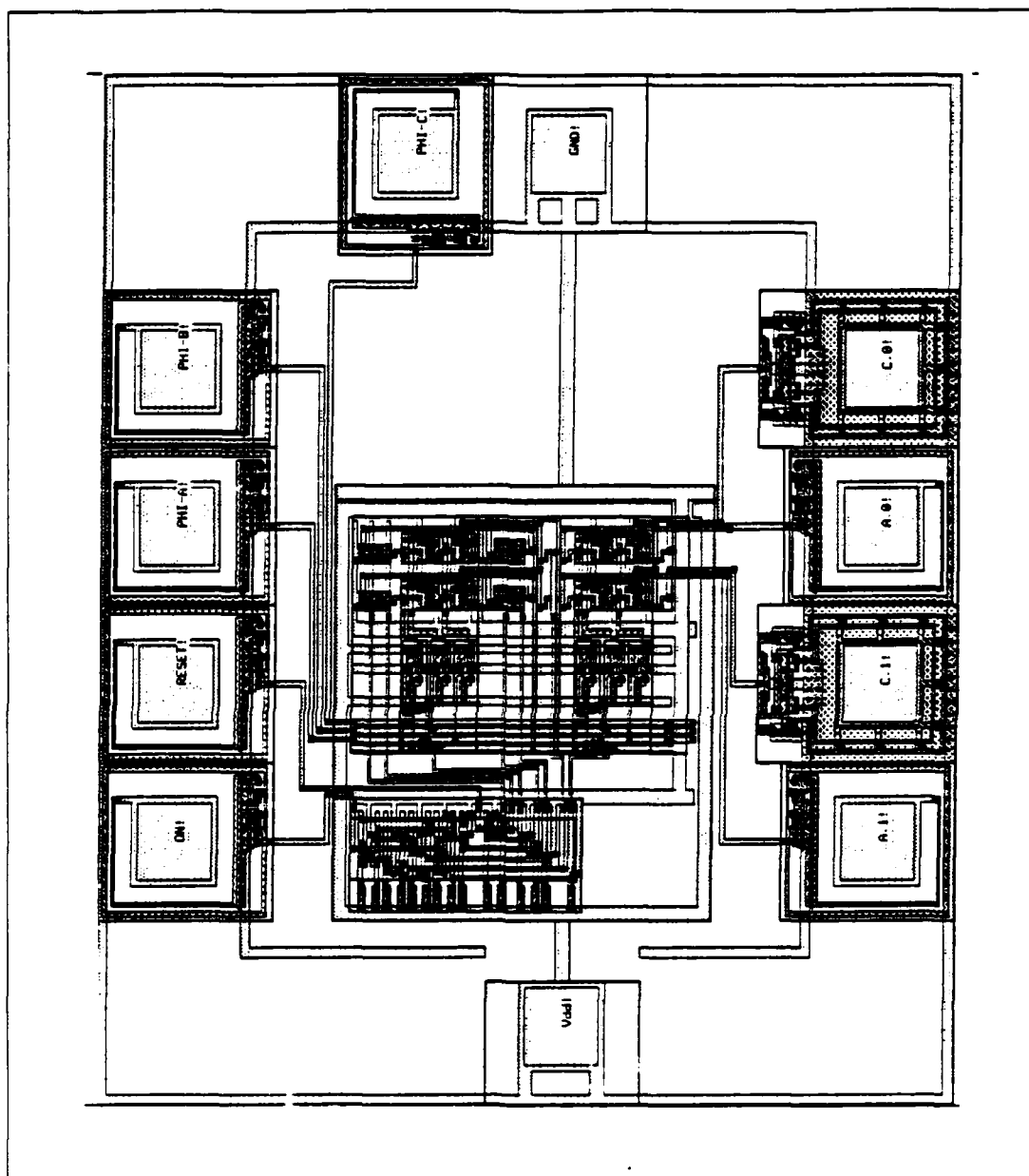
Figure 31: Placing pads on four sides.
