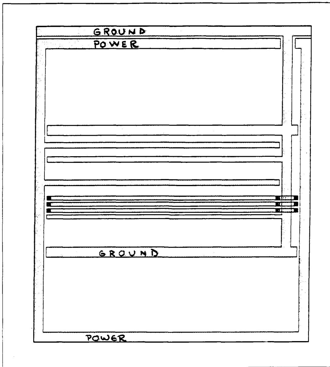
Figure 30: MacPitts' power and ground frame
