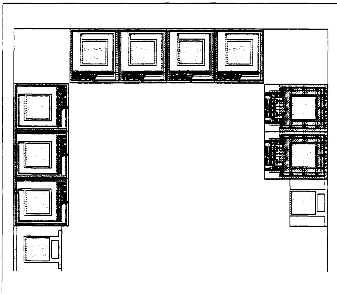
Figure 33: Pins-layout
