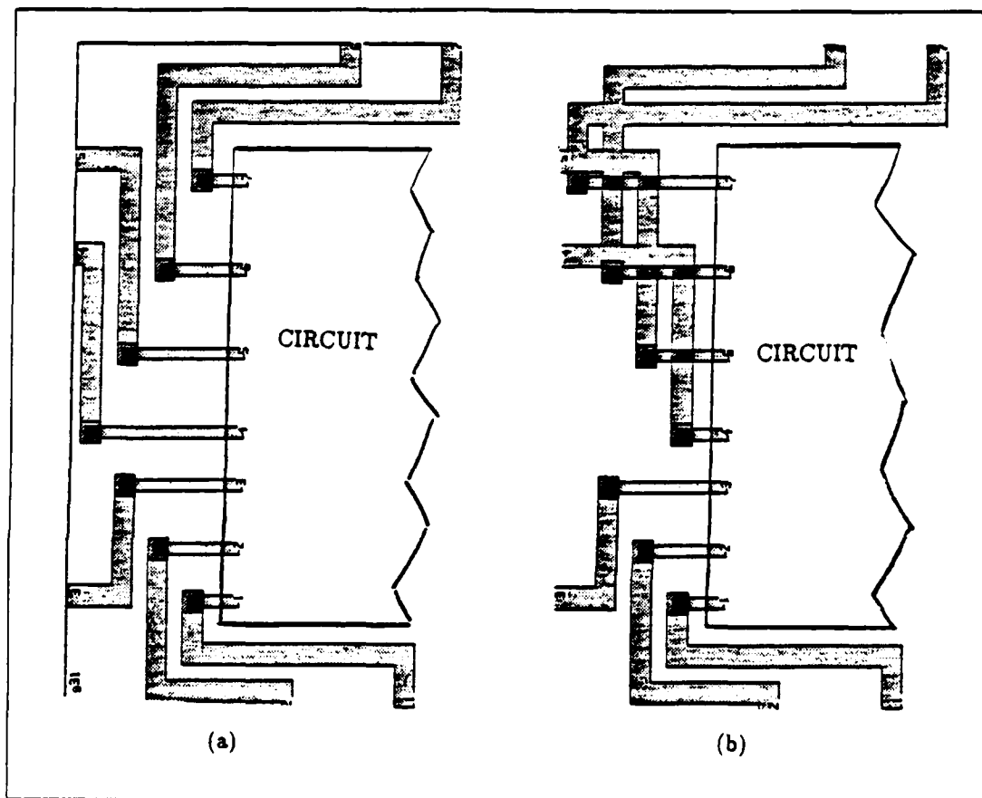
Figure 36: Sample routing problem: (a) routing by Monterey silicon compiler, (b) errors caused by change in routing direction
