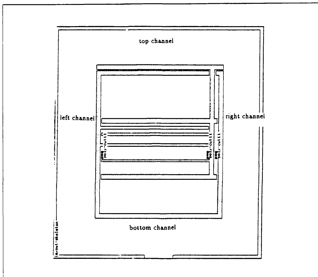
Figure 35: Pad routing area
