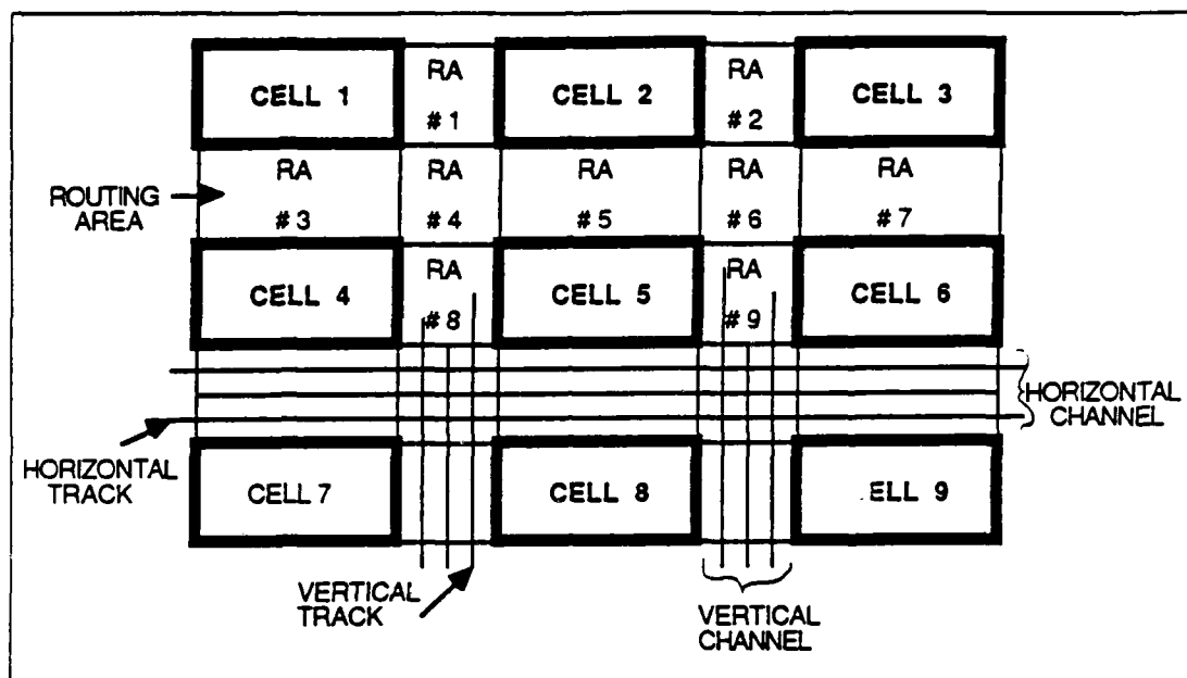
Figure 5: Partitioning a chip into global wiring cells.
