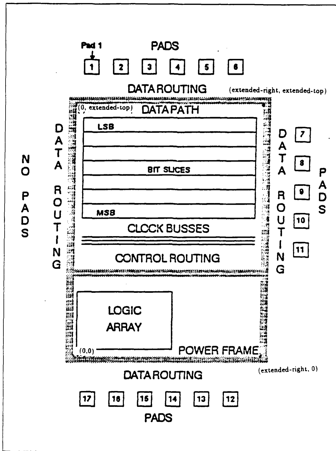
Figure 25: MacPitts floor plan.
