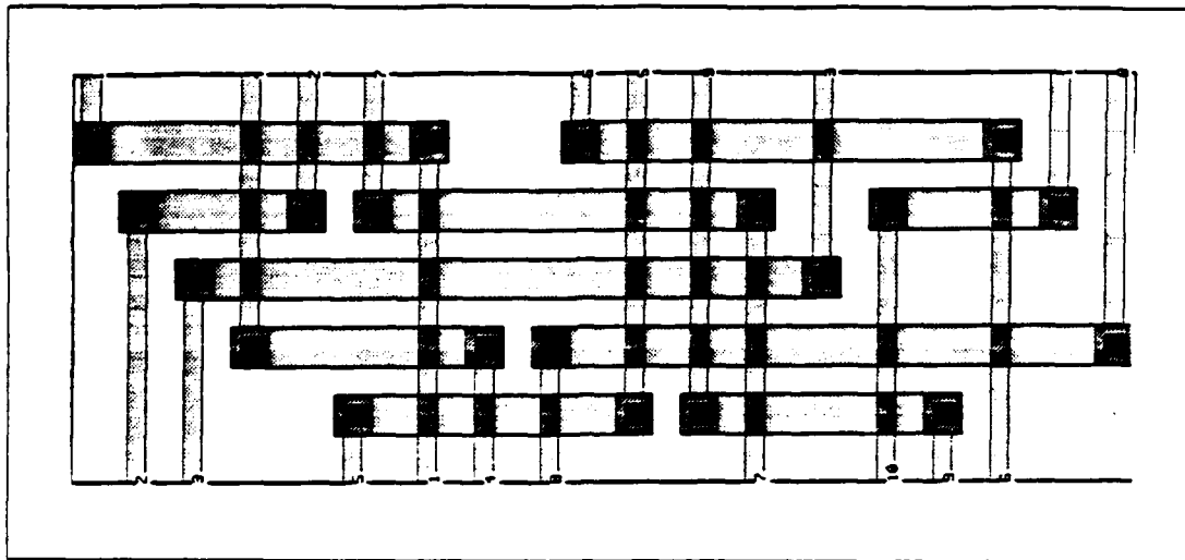
Figure 11: The left-edge channel router.
