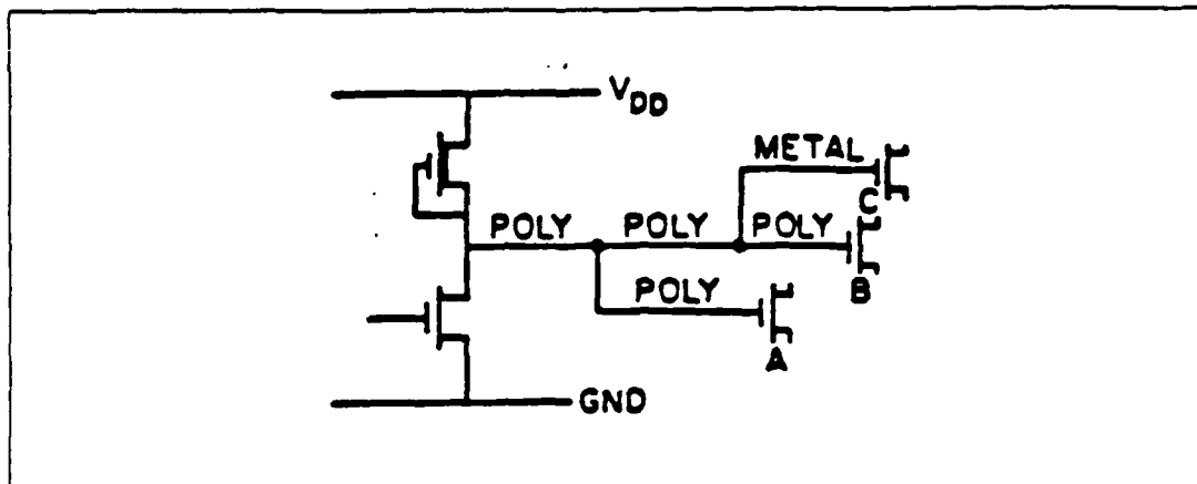
Figure 46: MOS inverter circuit with fanout
