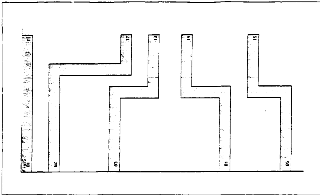
Figure 17: The river routing problem
