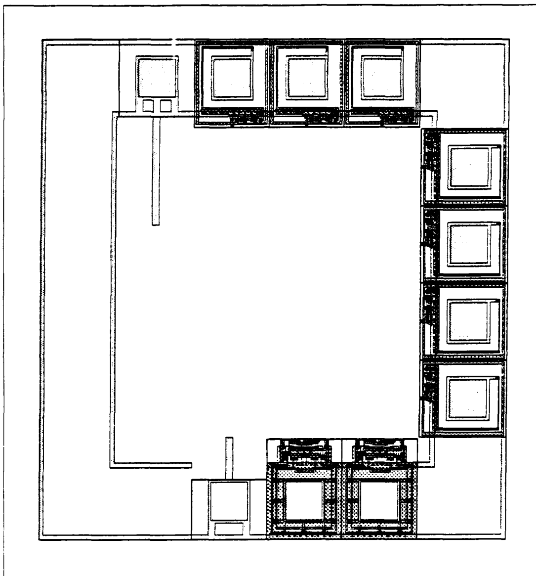
Figure 29: MacPitts' pad ring.
