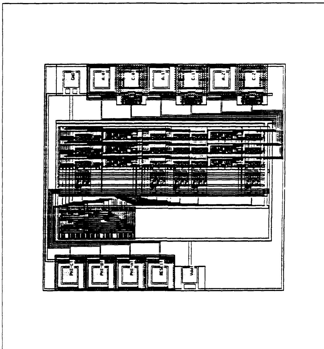
Figure 41: TEST circuit design by Monterey
