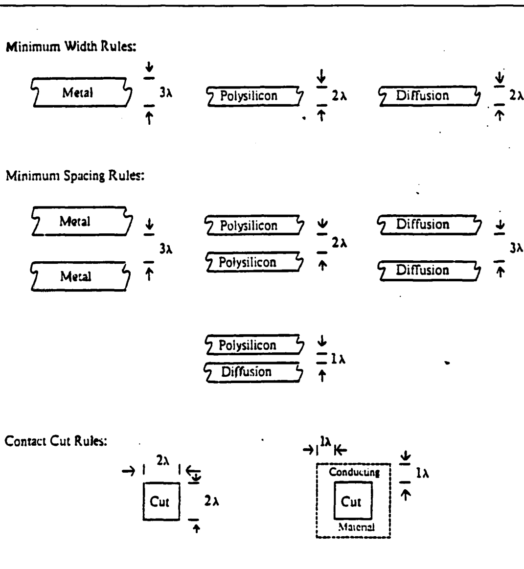
Figure 1: Mead-Conway width and spacing rules
