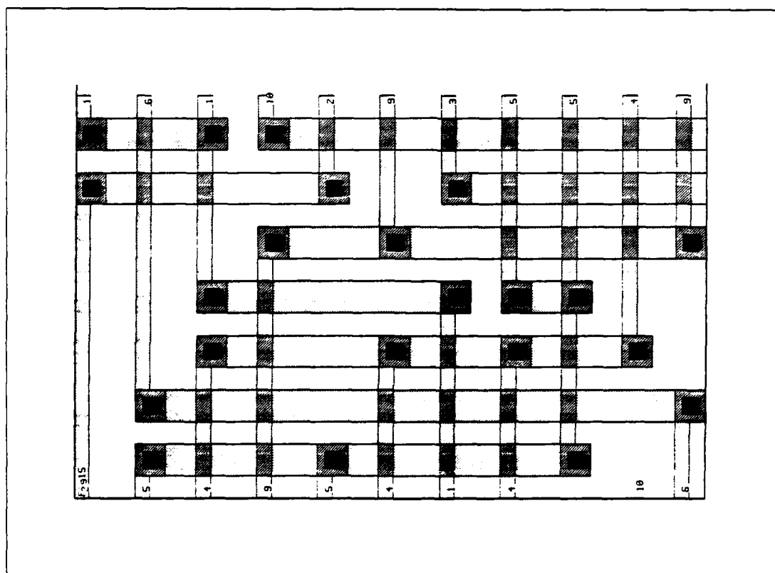
Figure 16: A channel unrouteable by the greedy algorithm.
