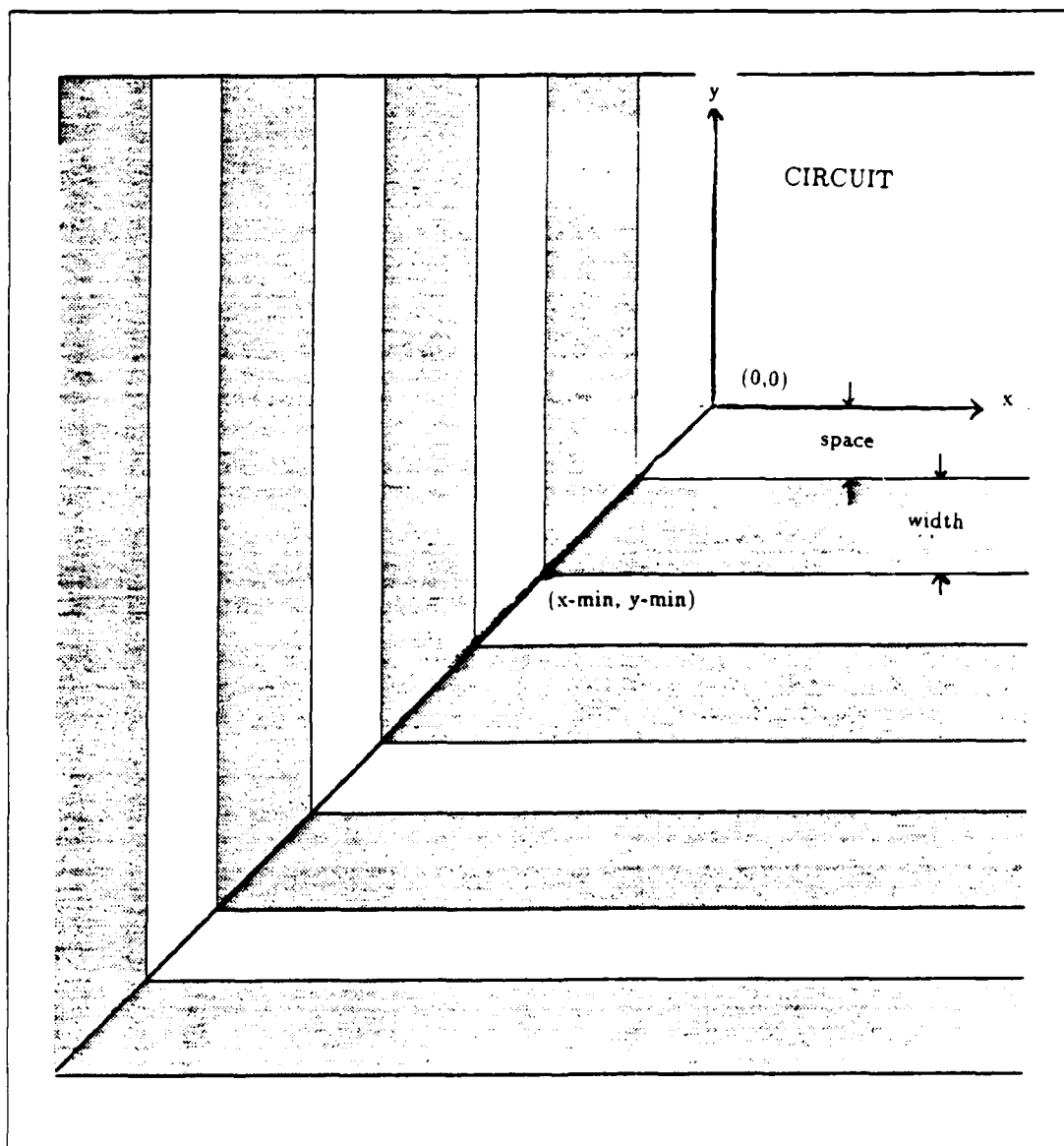
Figure 37: Routing the corners
