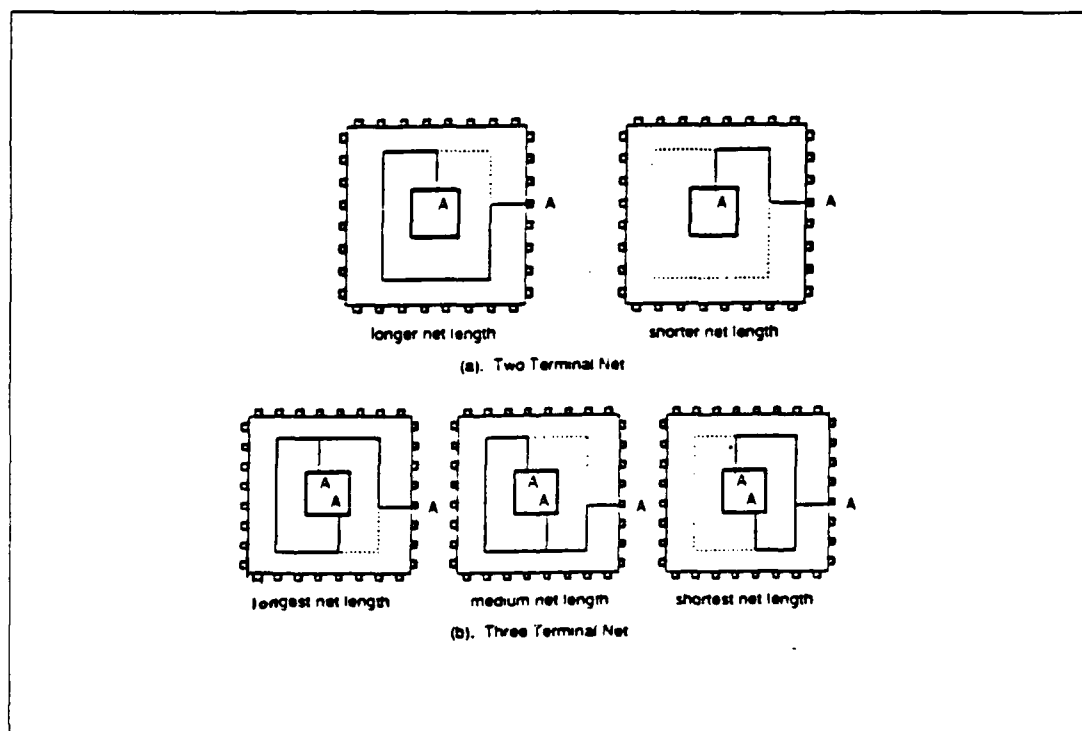
Figure 19: Moat routing direction ambiguity
