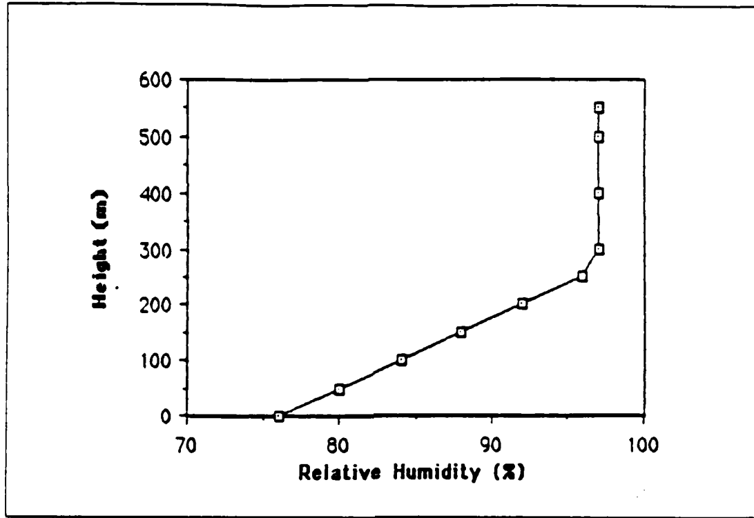
Fig. 6. Assumed relative humidity profile when layer relative humidity exceeds 97%.
