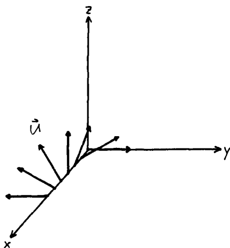
Figure 3.2: Example 1: Beltrami Wave
