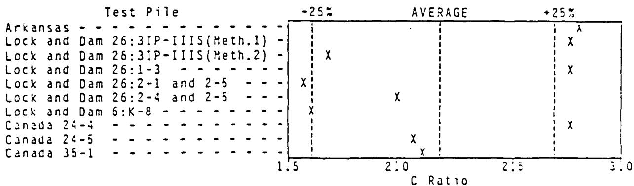
FIGURE 1. - Plot of C Ratios: Uncorrected for Residual Stress
