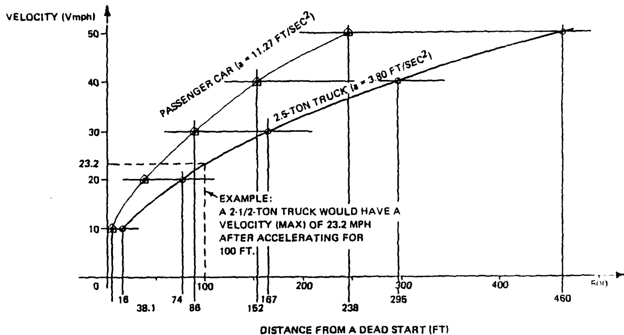
Figure 3.3: Vehicle Velocity (Terrorist Vehicle Bomb Survivability Manual, p.3-8)
