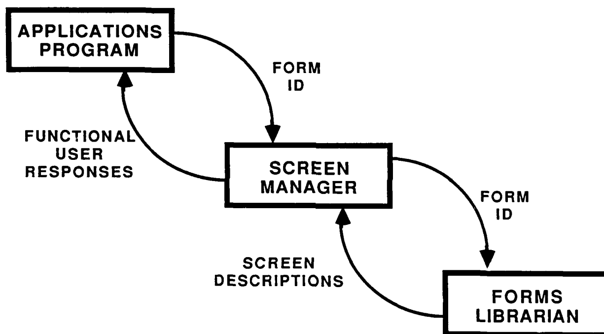
Figure 2. Data Flow
