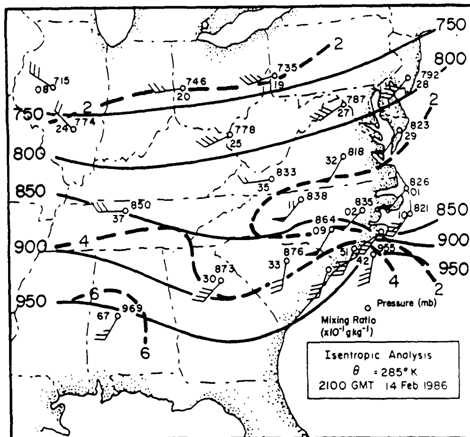
Figure 3.8a. Isentropic analyses of pressure, wind, and mixing ratio on the 285-K surface at 2100 GMT 14 February 1986: pressure (solid contours, mb); mixing ratio (heavy dashed, \text{g kg}^{-1} ); wind (barb = 5 \text{ m s}^{-1} , pennant = 25 \text{ m s}^{-1} ).
