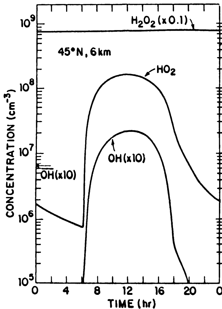
Figure 1. Modelled average mean values of odd hydrogen species free radicals emphasizing the expected diurnal variations in OH and HO 2 radicals [Logan et al., 1981].
