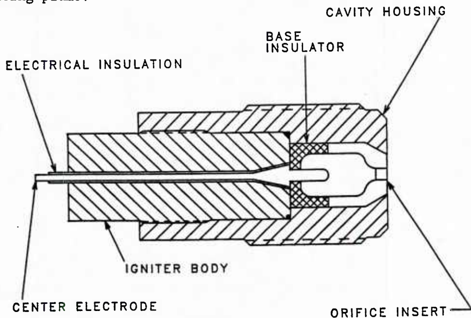
Figure 3. Electrical LP Igniter
