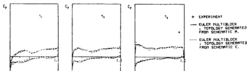
WING - BODY - CANARD COMPARISON OF TOPOLOGIES M=1.2 \alpha=6.00
