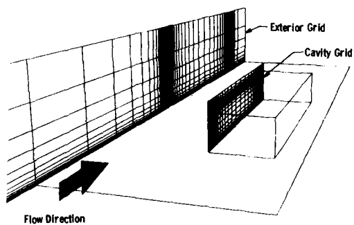
Fig. 10. Computational Grids.
