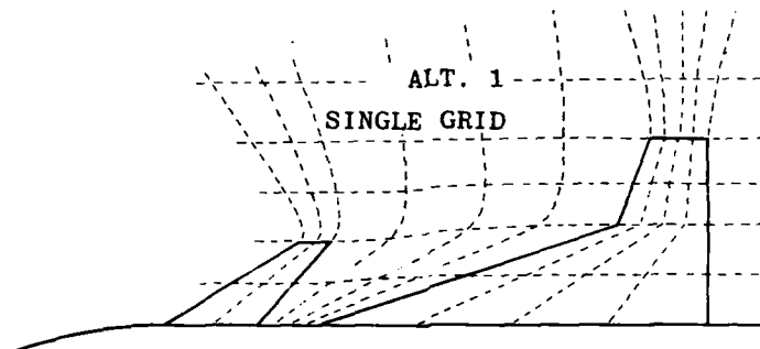
Figure 5.- Topology for a Single-Block Grid with Grid-Line Alignment with Lifting Surfaces.
