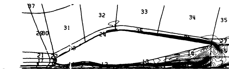
Figure 23: Total Pressure Loss Contours.
