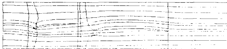
FIGURE 4. GRID STRUCTURE ON THE BODY DERIVED FROM GEOMETRICAL SCHEMATIC A.
