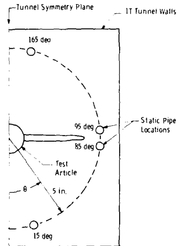
Fig. 6. Schematic of Mobile Static Pipe Locations in Tunnel IT.
