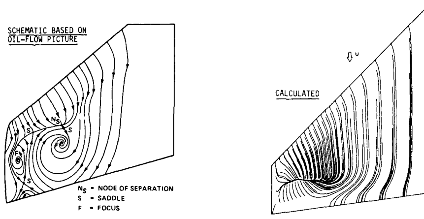
Figure 5. Comparison of the Skin Friction Lines ( 45^\circ -Sweep Wing).
