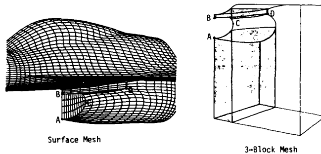
Figure 6. Mesh for the F-16 (Ref. 10).
