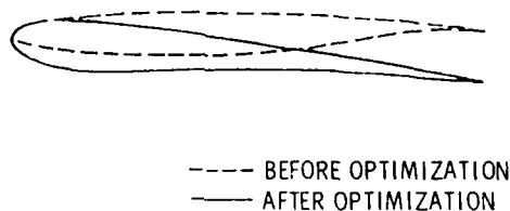
Fig. 2.3 Optimal Airfoil
