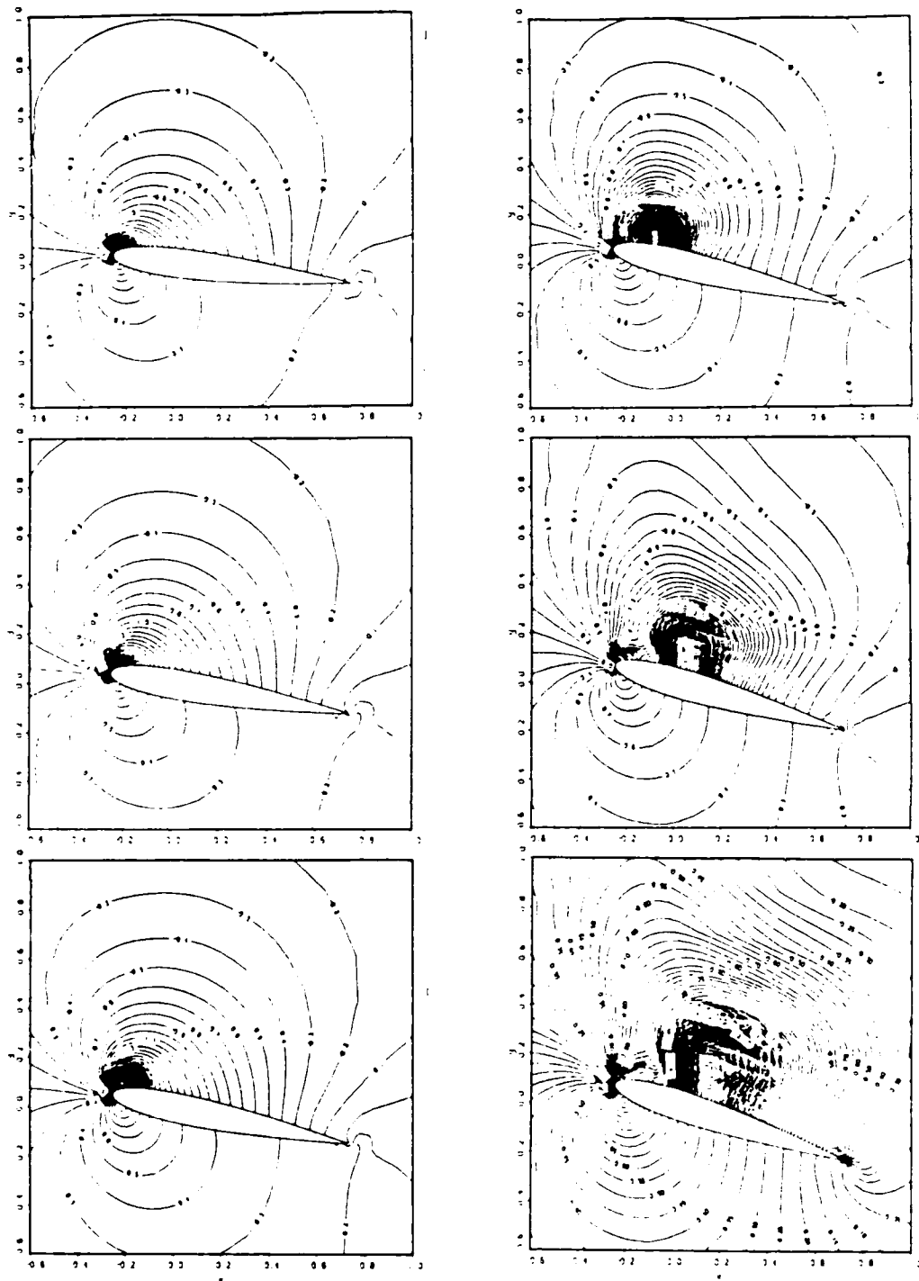
Figure 4. Pressure Contours, \alpha = 15^\circ - 10^\circ (.151t) , \alpha = 12.20^\circ, 14.30^\circ, 16.43^\circ, 18.50^\circ, 20.40^\circ, 22.07^\circ , (top to bottom, left to right), M_\infty = .283 , Re = 3.45 \times 10^6 , \eta_{min} = .00005 .
