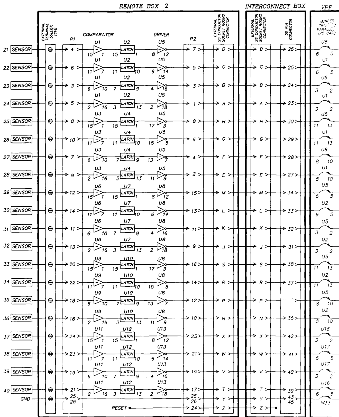
Figure C-2. MDDS channel interconnection diagram.
