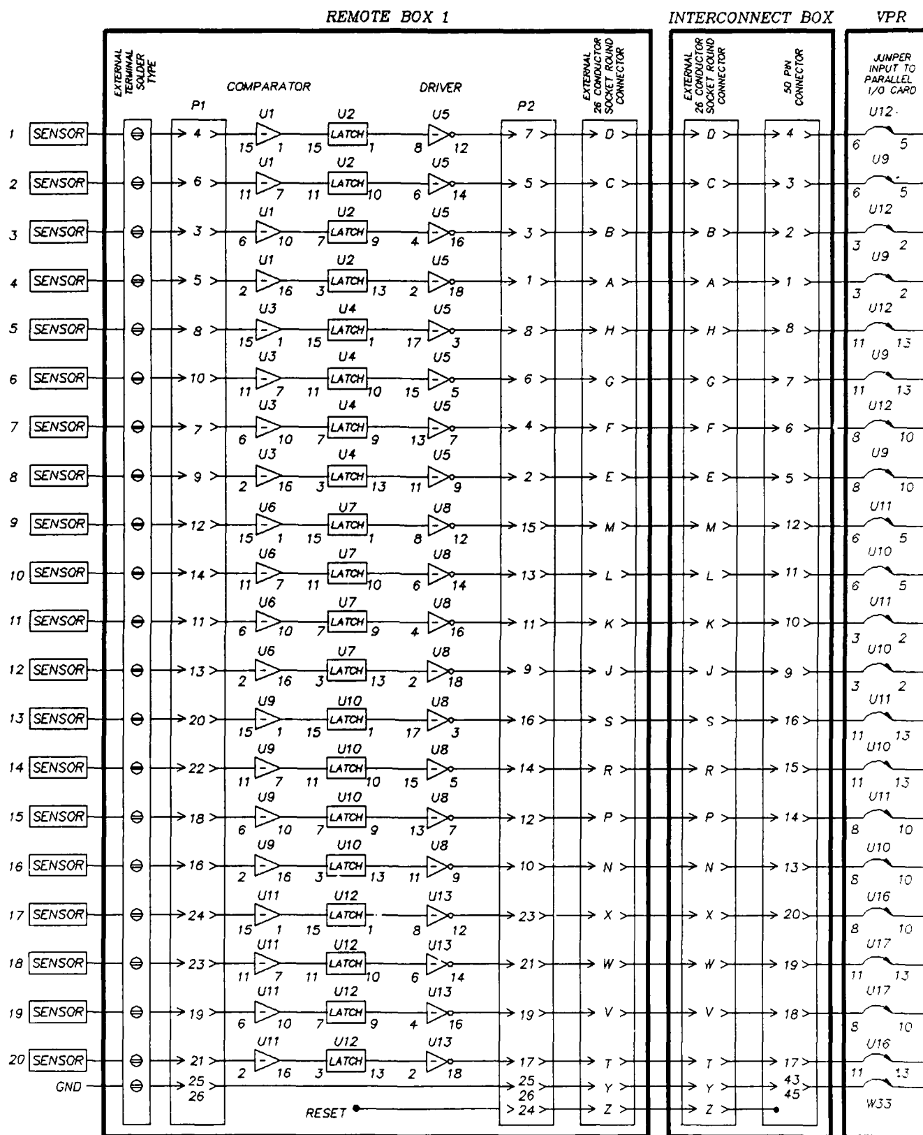
Figure C-1. MDDS channel interconnection diagram.
