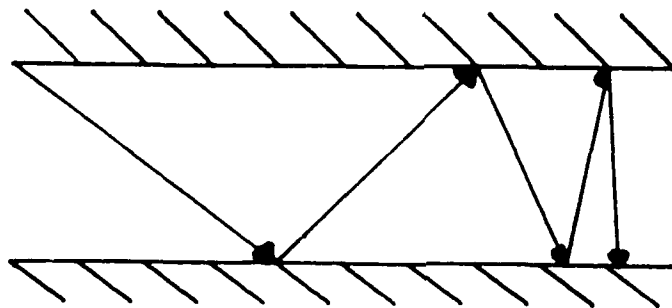
Figure (4.7) - Electromagnetic Radiation in a Waveguide with Spatially Dependent Permittivity
