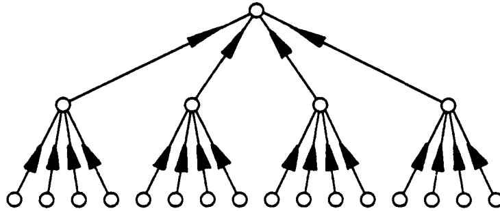
Figure 5.5: Combining messages
