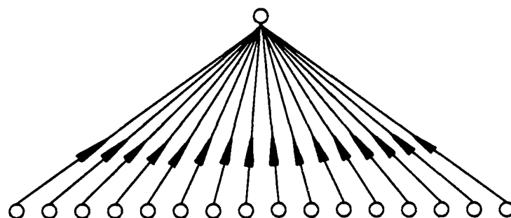
Figure 5.4: Concurrent write
