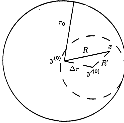
Figure 3.4: Lemma 3.2.3
