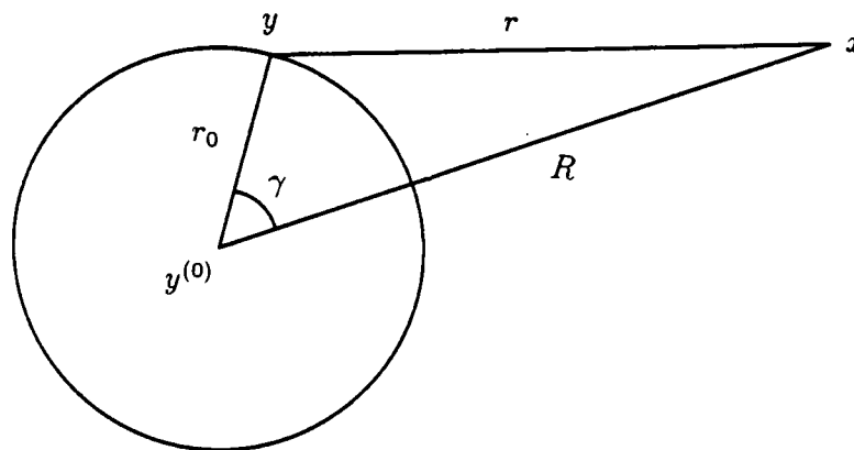
Figure 3.1: Gravitational field
