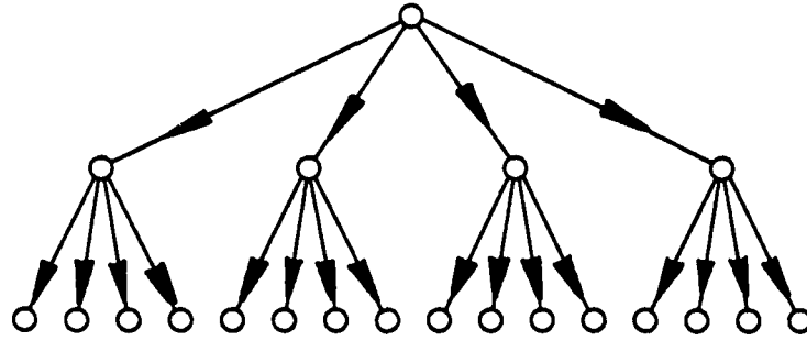
Figure 5.6: Delegating messages
