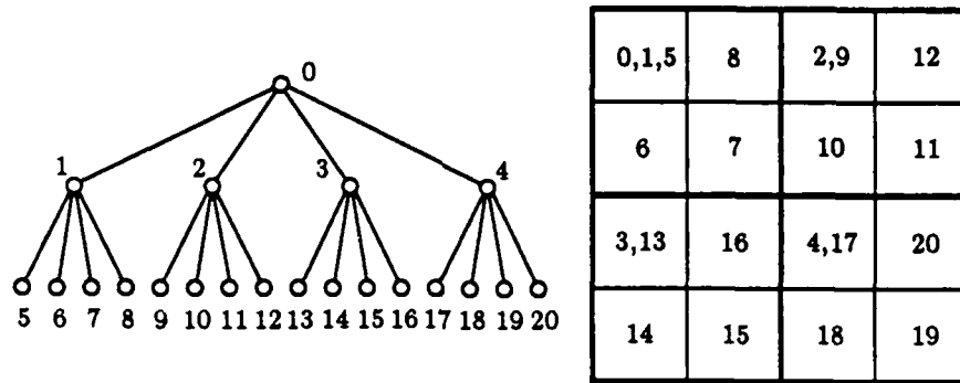
Figure 5.7: Superimposed mapping. Each square in the grid represents a processor, and each number represents a node in the tree.
