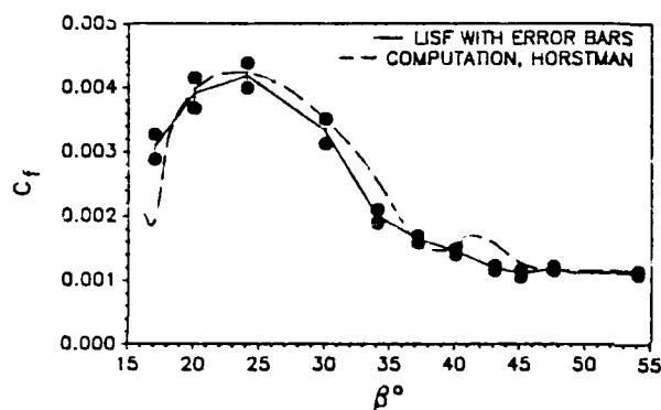
Fig. 7 - c_f Distribution for \alpha = 16^\circ with CFD Comparison.
