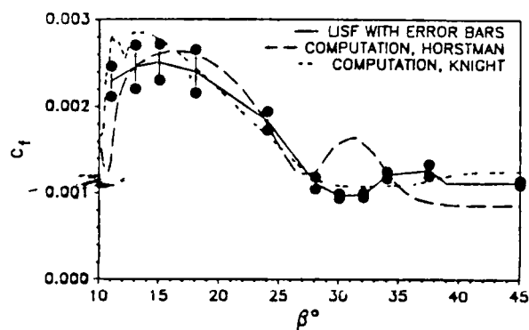
Fig. 6 - c_f Distribution for \alpha = 10^\circ with CFD Comparisons.
