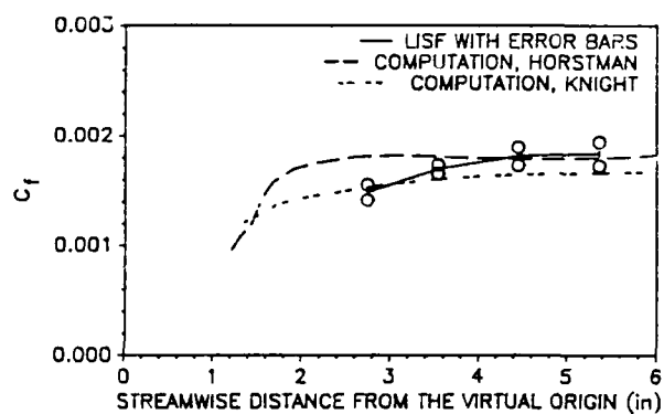
Fig. 8a - c_f Distribution Along \beta = 24^\circ Conical Ray for \alpha = 10^\circ .
