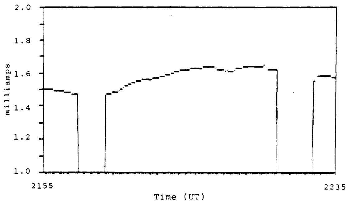
Figure 17. Ion gun beam current.
