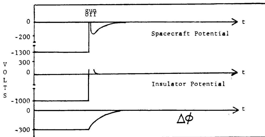
Figure 37. Spacecraft and insulator potential.
