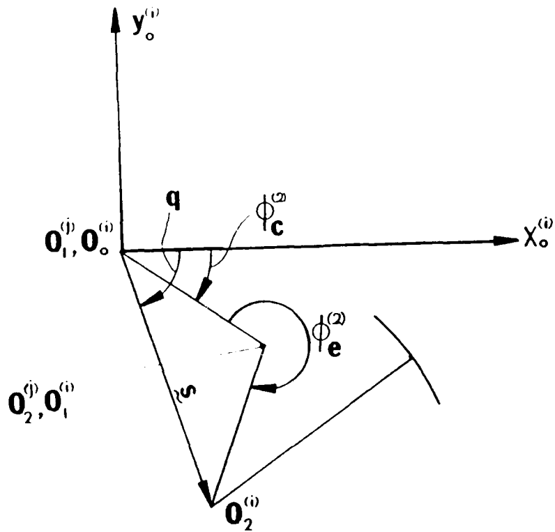
Fig. 3.1 Basic Settings for Left-Hand Pinion
