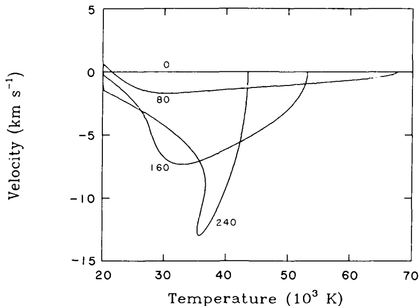
FIG. 7.—Plots of velocity versus temperature at times of 0, 80, 160, and 240 s during the cooling tall loop simulation of Fig. 6.
