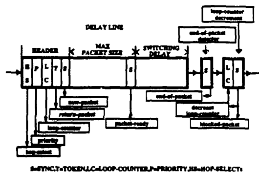
Figure 19: Delay Line with loop-counter implementation
