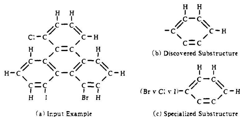
Figure 1. SUBDUE Example
