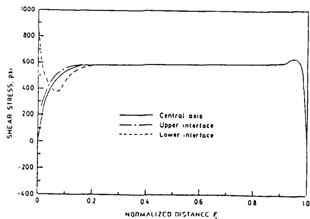
FIG. 23 Stress Distributions in an LBAST Specimen with Sharp Adherends
