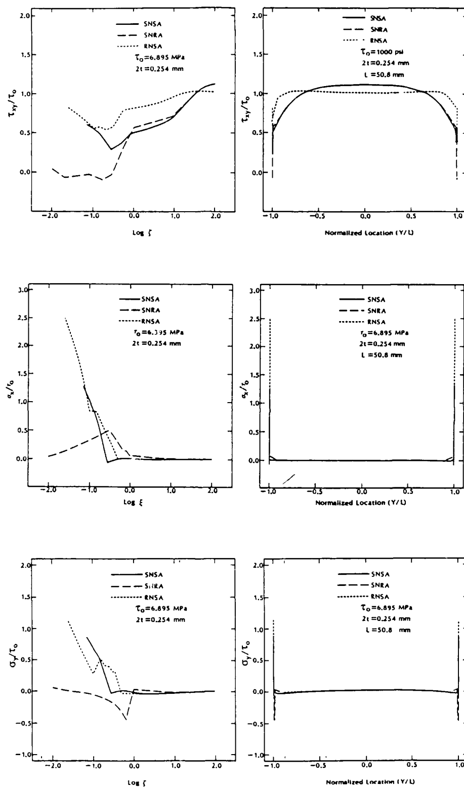
FIG. 10 Stresses in a Stiff Adherend Specimen Under Shear Loading
