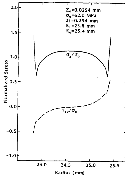
FIG. 2 Napkin Ring Specimen Under Bond-Normal Loading
