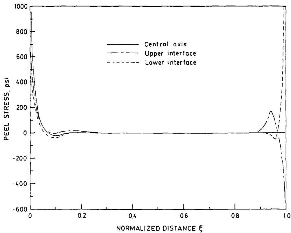
FIG. 24 Stress Distributions in an LBAST Specimen With Rounded Adherends
