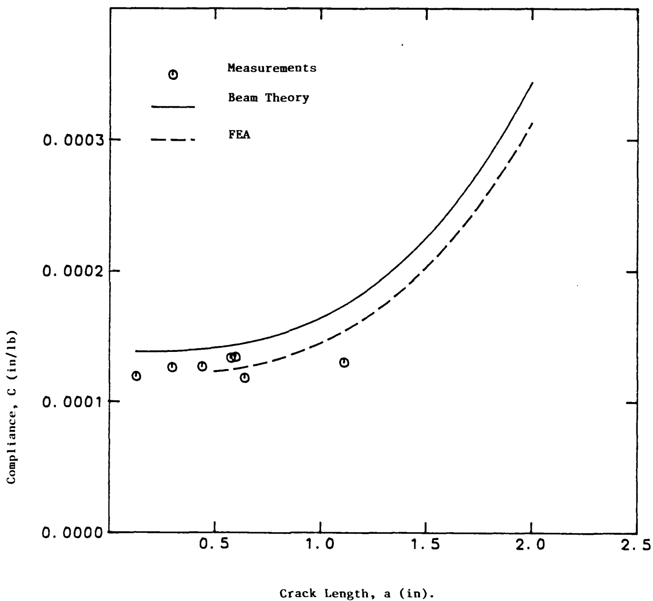
FIG. 41 Compliance of Cracked Ti - FM36 ENF Specimens
