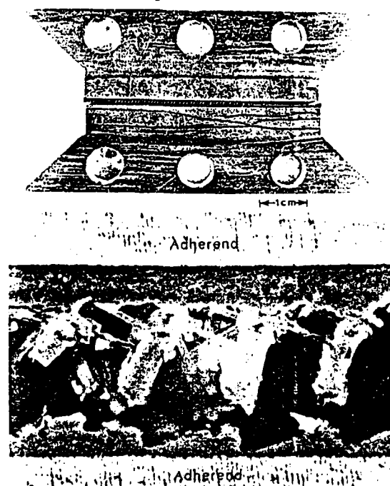
FIG. 19 Fracture Surfaces of a Modified Stiff Adherend Specimen (SNRA) Tested Under Pinned Boundary Conditions
