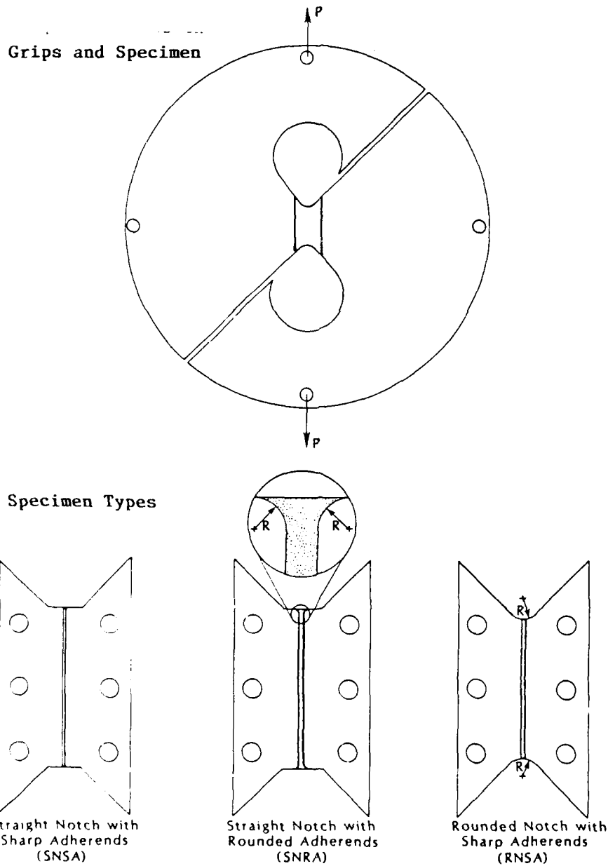
FIG. 9 Stiff Adherend Specimen
