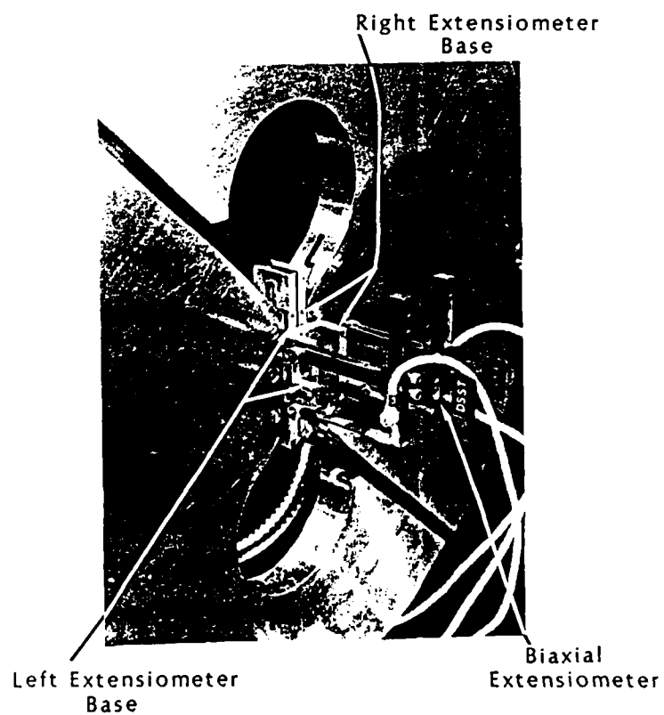
FIG. 15 Extensometer Mounting
