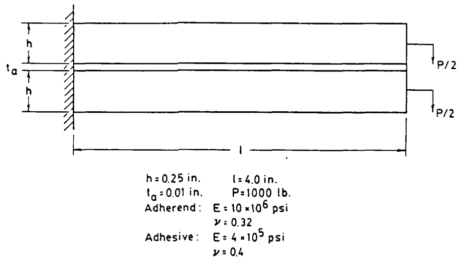
FIG. 21 Bending Laminated Beam Adhesive Shear Test (LBAST) Specimen Geometry
