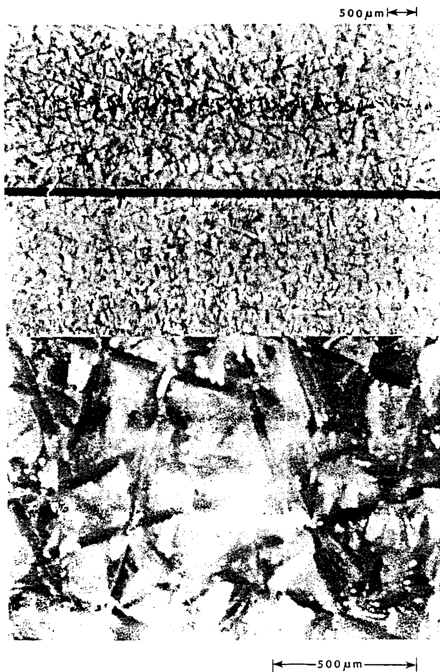
FIG. 17 Fracture Surfaces of a Modified Thick Adherend Specimen (SNRA) Tested Under Clamped Boundary Conditions
