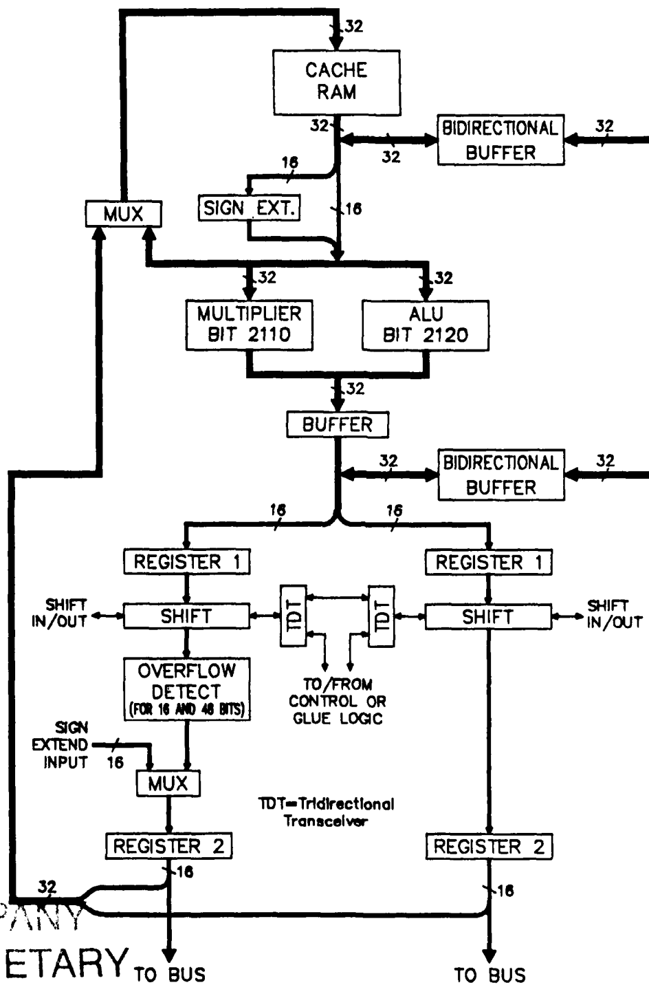
Figure 21. Architecture Using a High-Speed ALU-Multiply Chip Set with Multiply and Divide.
