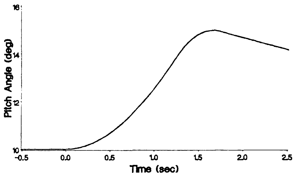
Figure 78. Linear Optimal Control Law in Full System Simulation
