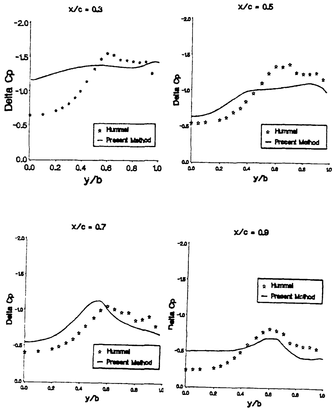
Figure 37. Steady State Pressure Distribution
