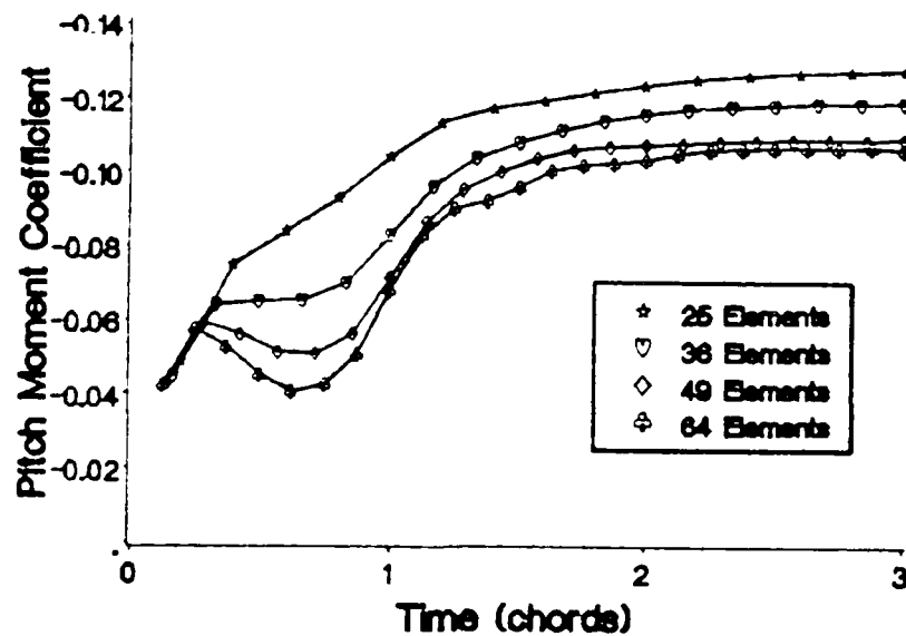
Figure 34. Pitch Moment Coefficient as Number of Elements is Increased
