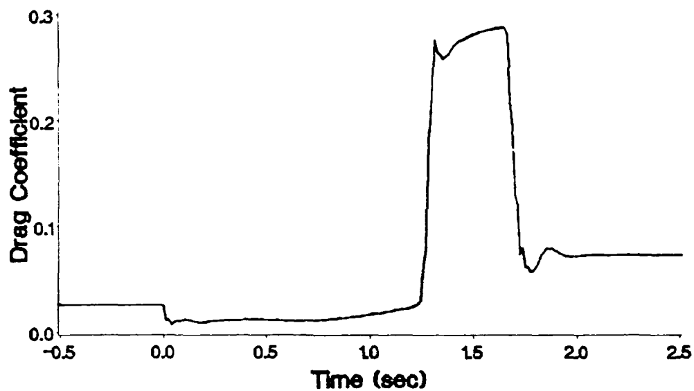
Figure 82. Optimal Control Drag Coefficient
