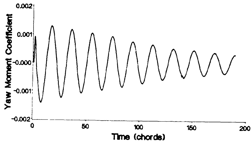
Figure 97. Feedback System Yaw Moment Coefficient
