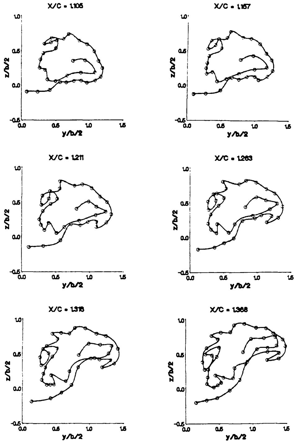
Figure 40. Vortex Sheet Location Downstream of the Wing
