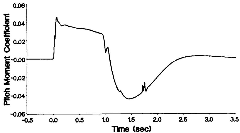
Figure 90. Feedback Control Pitch-Moment Coefficient
