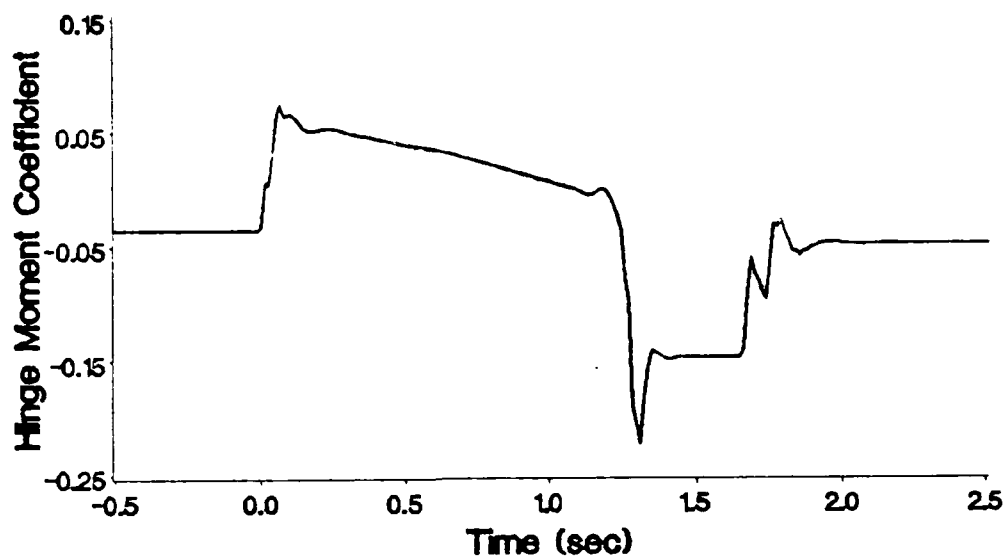
Figure 84. Optimal Control Hinge Moment Coefficient
