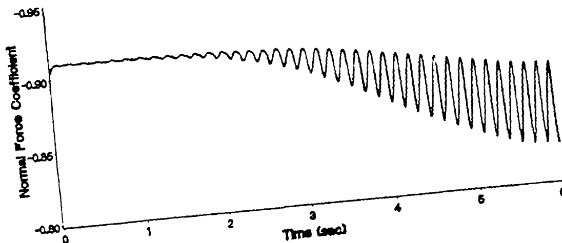
Figure 65. Normal Force Evolution for a Pitch Angle of 27.5 Degrees
