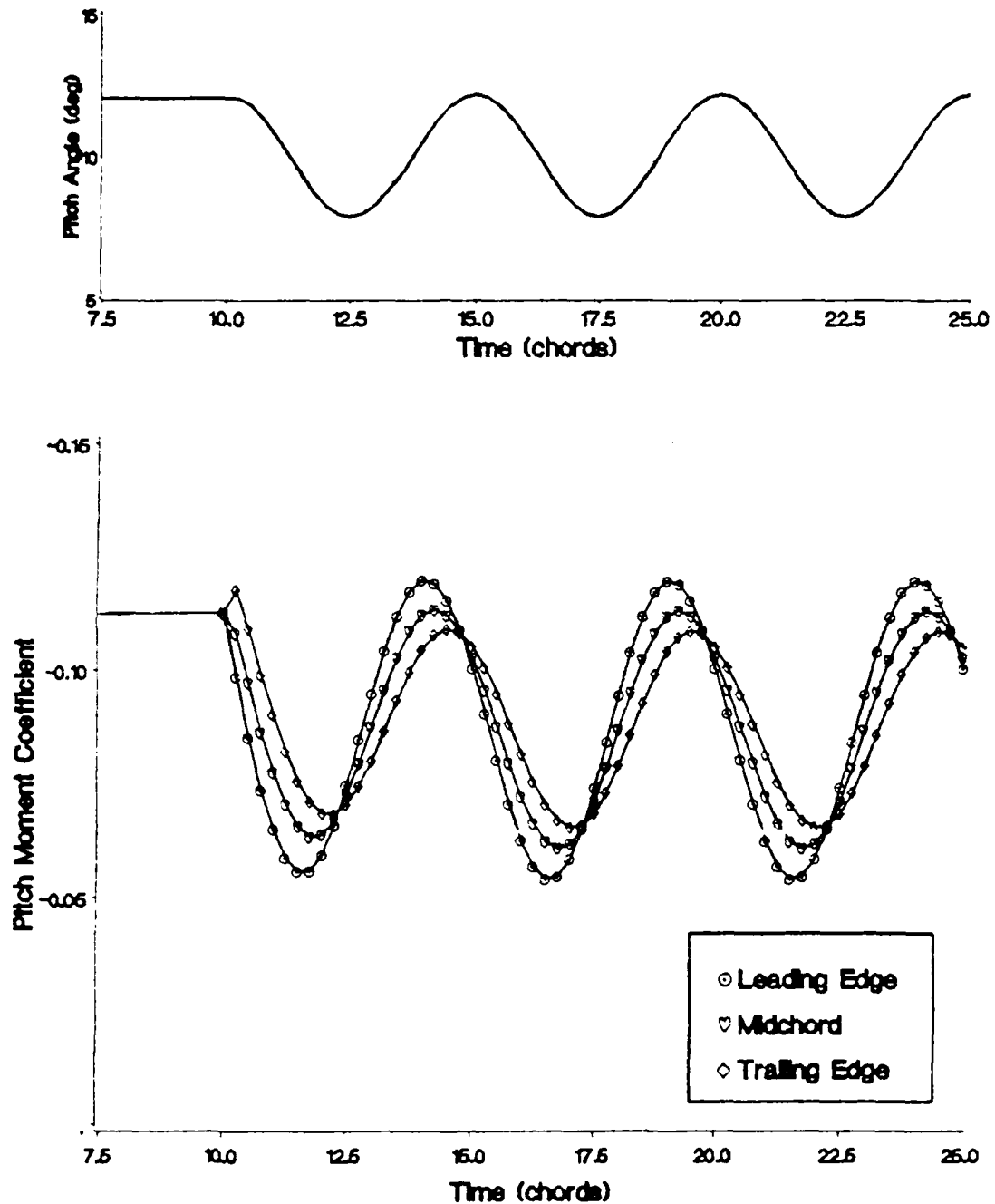
Figure 50. Pitch Moment as a Function of Time for Various Axes of Rotation
