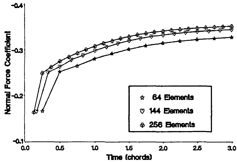
Figure 26. Normal Force Coefficient as Number of Elements is Increased
