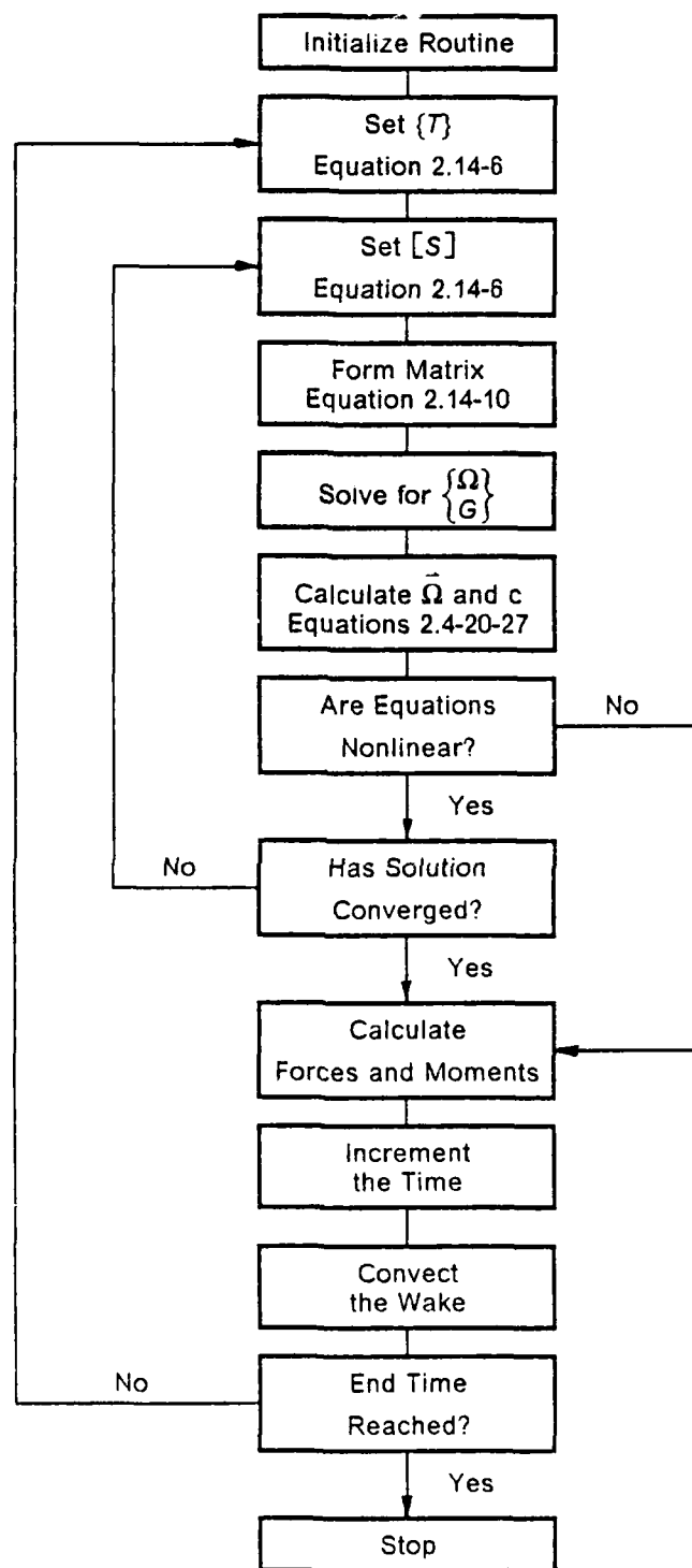
Figure 24. Flow Chart for the Aerodynamic Model
