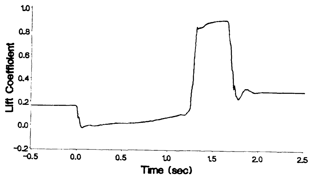
Figure 81. Optimal Control Lift Coefficient
