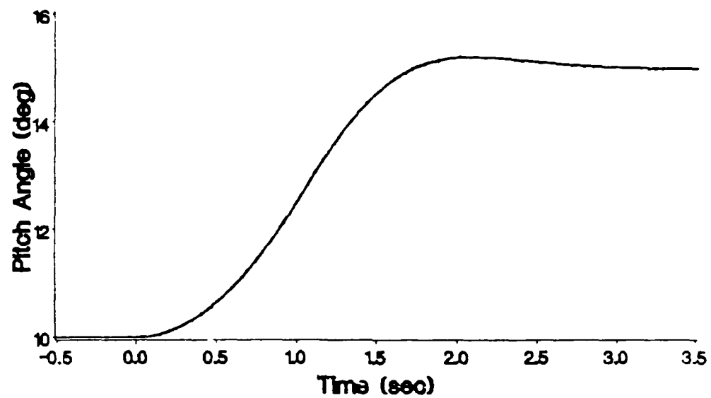
Figure 86. Feedback Control Pitch Angle
