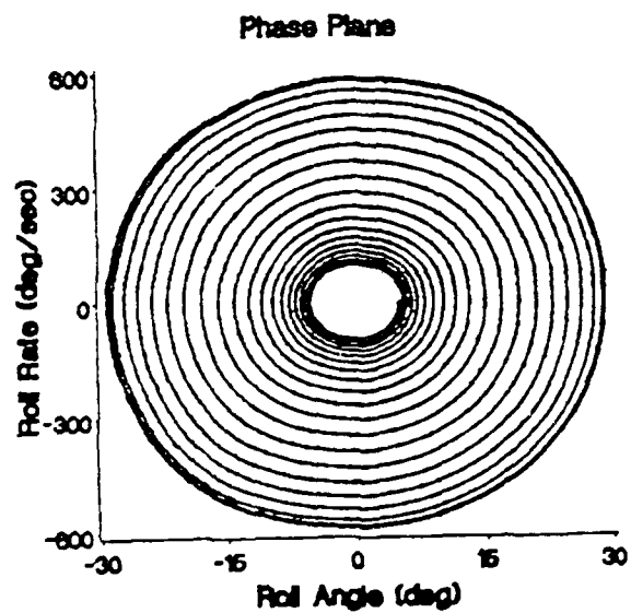
Figure 64. Phase Portrait for a Pitch Angle of 27.5 Degrees
