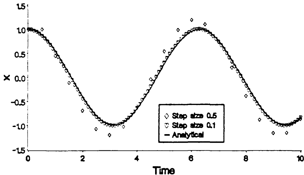
Figure 44. Validation of Numerical-Integration Scheme
