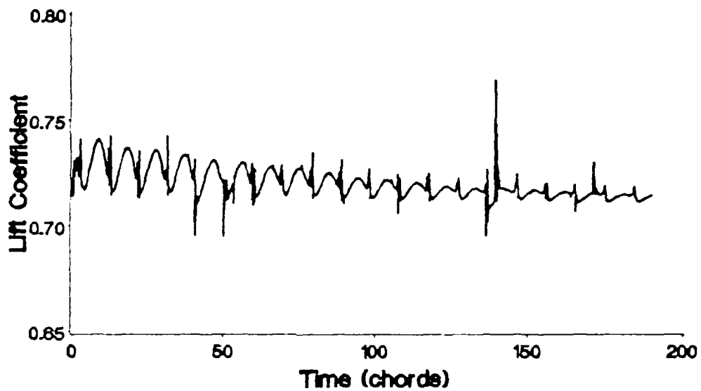
Figure 95. Feedback System Lift Coefficient
