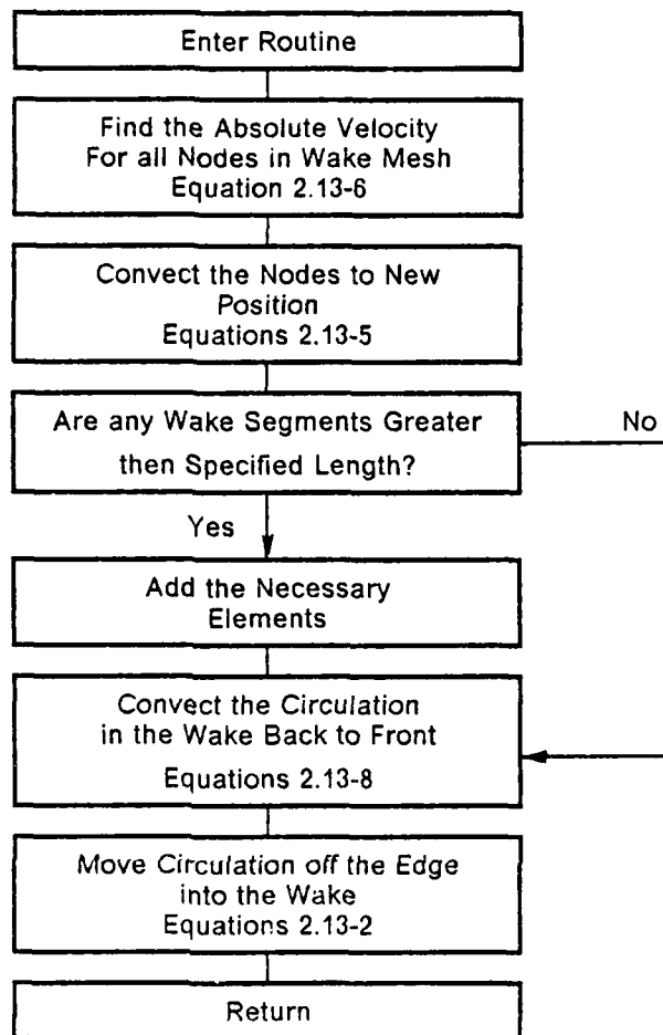
Figure 23. Flow Chart for Convecting the Wake
