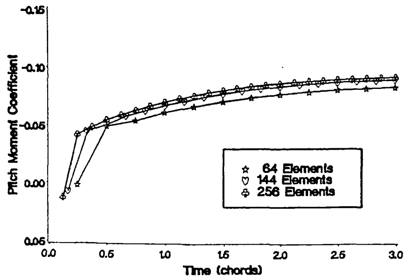
Figure 27. Pitch Moment Coefficient as Number of Elements is Increased
