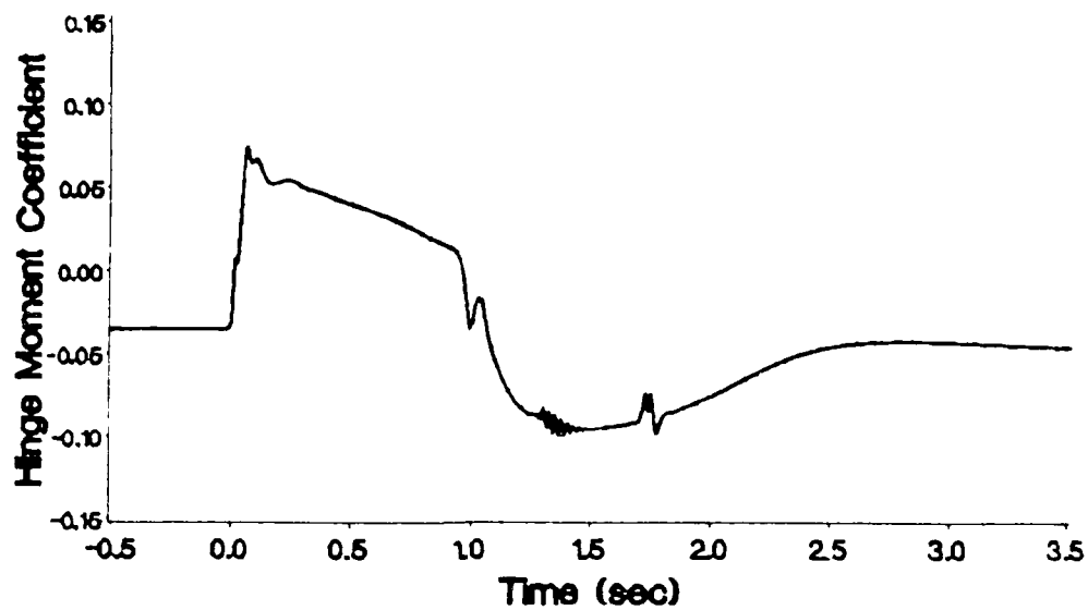
Figure 91. Feedback Control Hinge-Moment Coefficient
