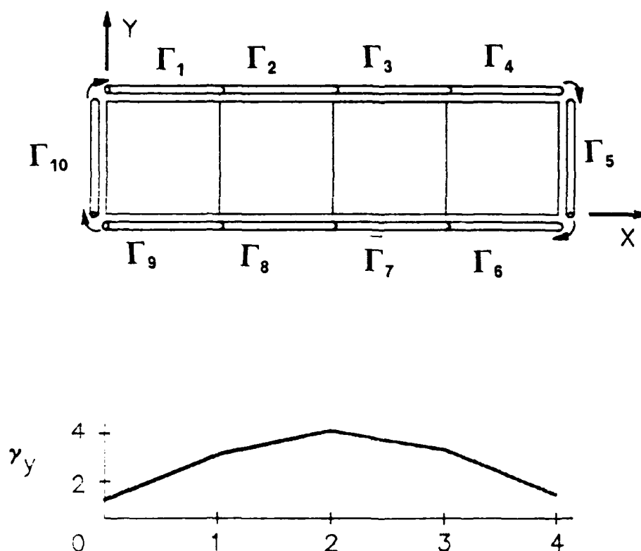
Figure 20. Test Configuration of A Vortex Sheet
