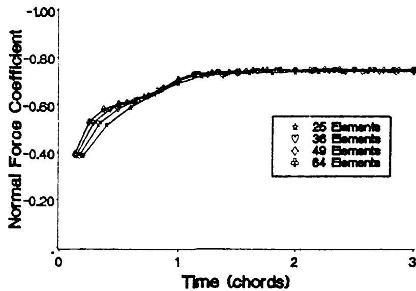
Figure 33. Normal Force Coefficient as Number of Elements is Increased
