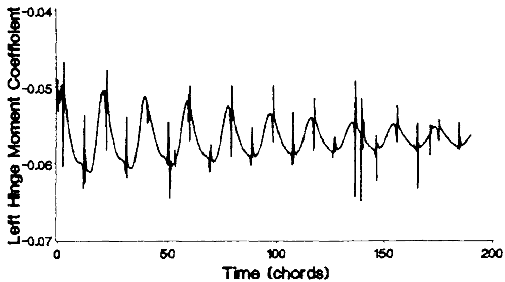
Figure 99. Feedback System Port Hinge Moment Coefficient
