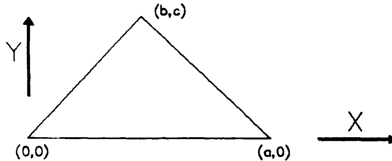
Figure 1. Triangular Element and Local Coordinate System
