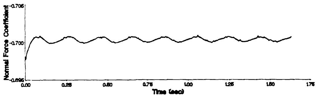
Figure 60. Normal Force Evolution for a Pitch Angle of 22.5 Degrees
