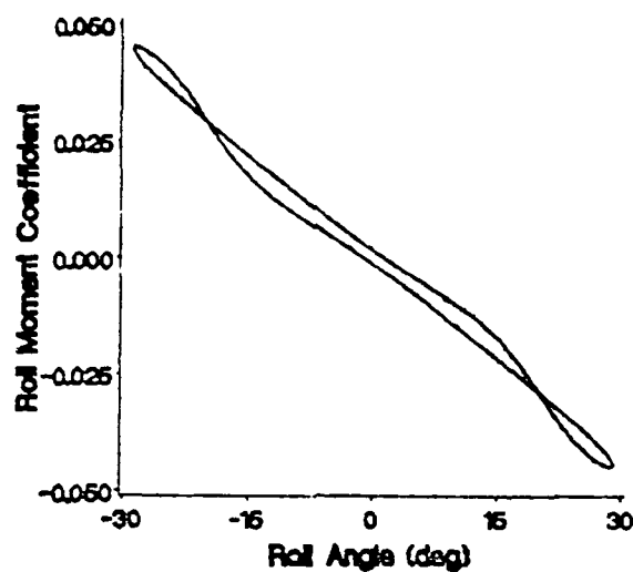
Figure 67. Roll Moment Hysteresis for a Pitch Angle of 27.5 Degrees
