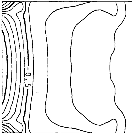
Figure 30. Steady State Pressure Distribution 10 Degrees Angle of Attack
