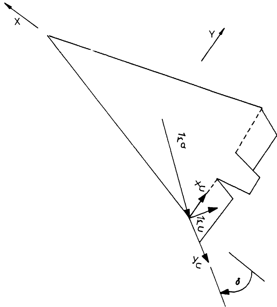
Figure 68. Control Surface Coordinate Frames
