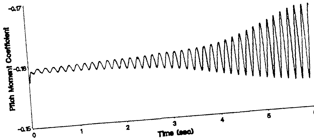
Figure 66. Pitch Moment Evolution for a Pitch Angle of 27.5 Degrees
