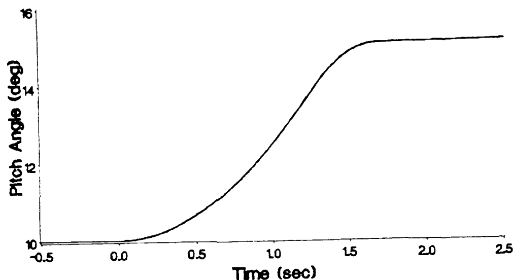
Figure 79. Optimal Control Pitch Angle
