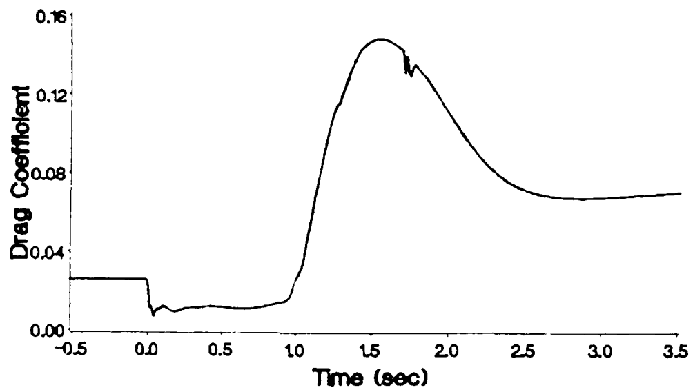
Figure 89. Feedback Control Drag Coefficient
