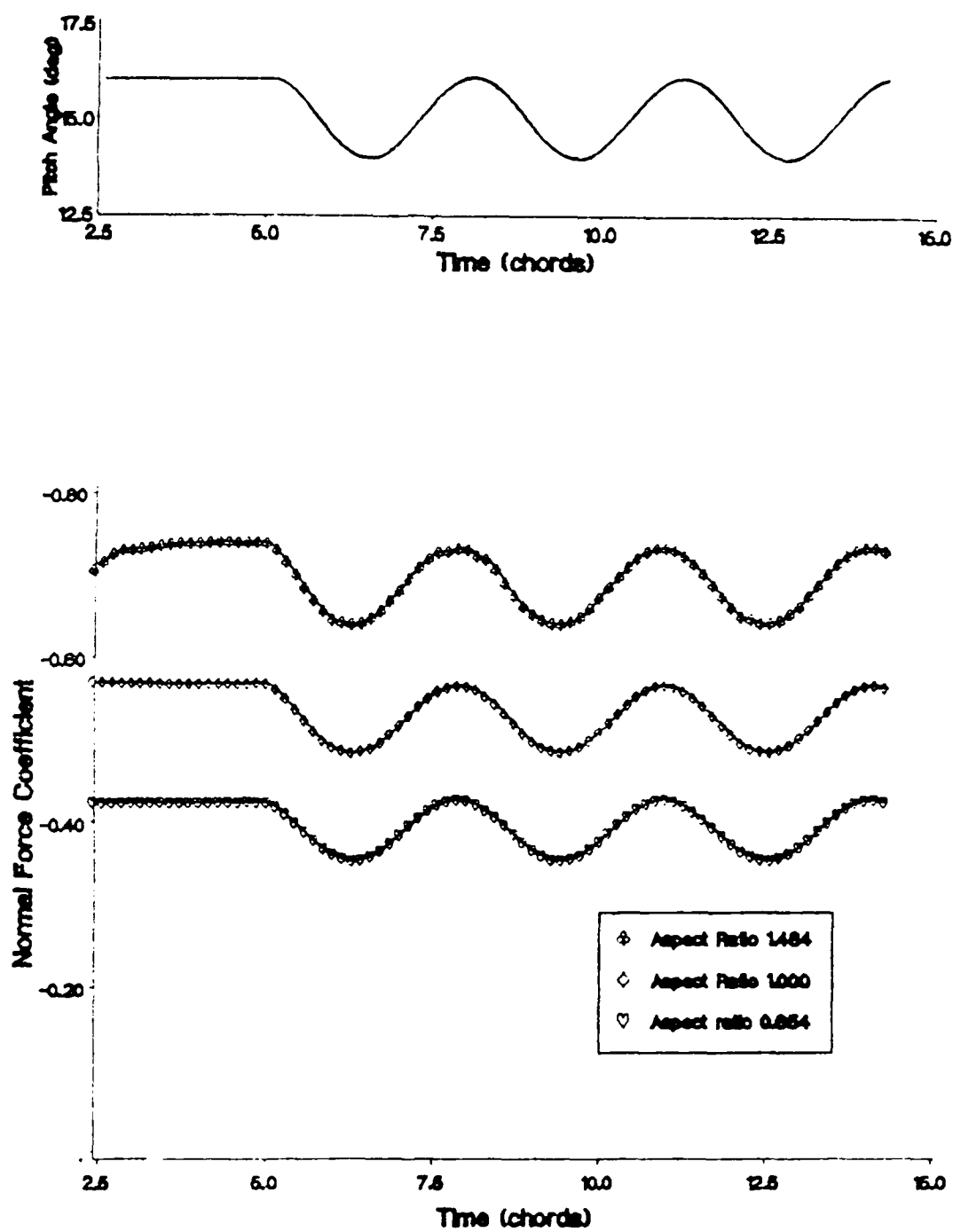
Figure 53. Normal Force as a Function of Time for a Reduced Frequency of 1.01
