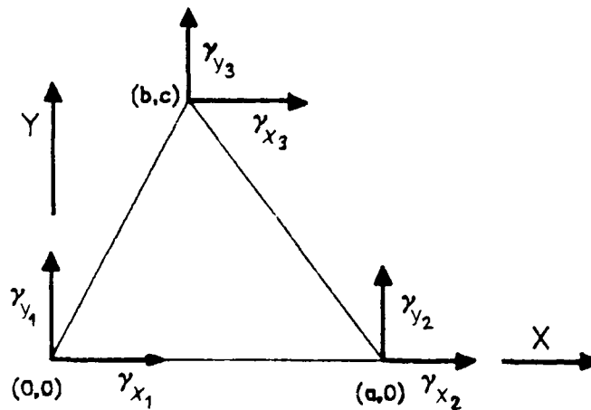
Figure 15. Triangular Element with Vorticity
