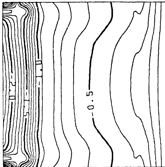
Figure 31. Steady State Pressure Distribution 20 Degrees Angle of Attack
