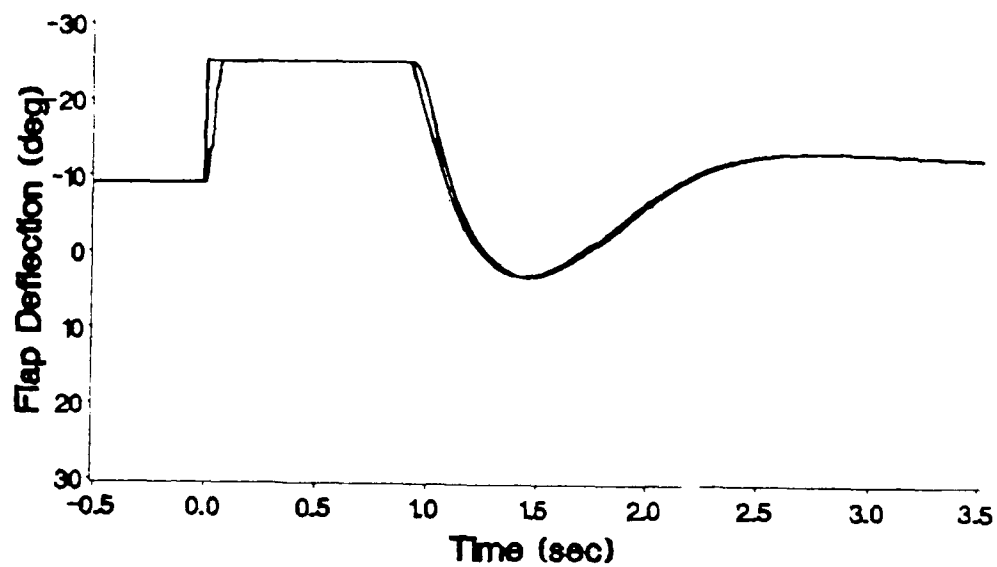
Figure 87. Feedback Control Flap Deflection
