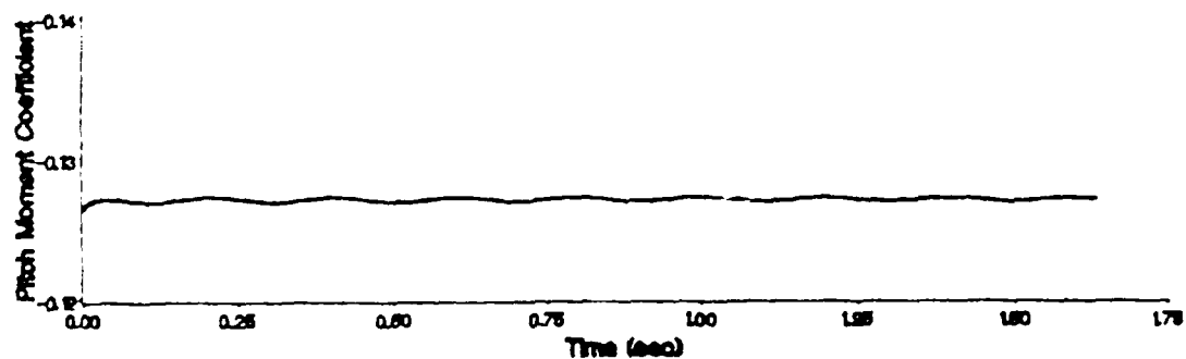
Figure 61. Pitch Moment Evolution for a Pitch Angle of 22.5 Degrees
