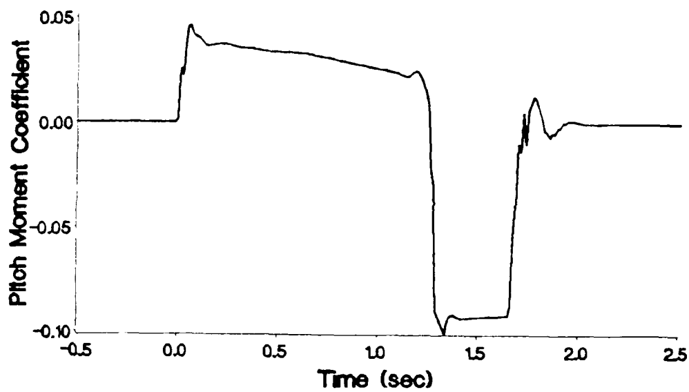
Figure 83. Optimal Control Pitch Moment Coefficient
