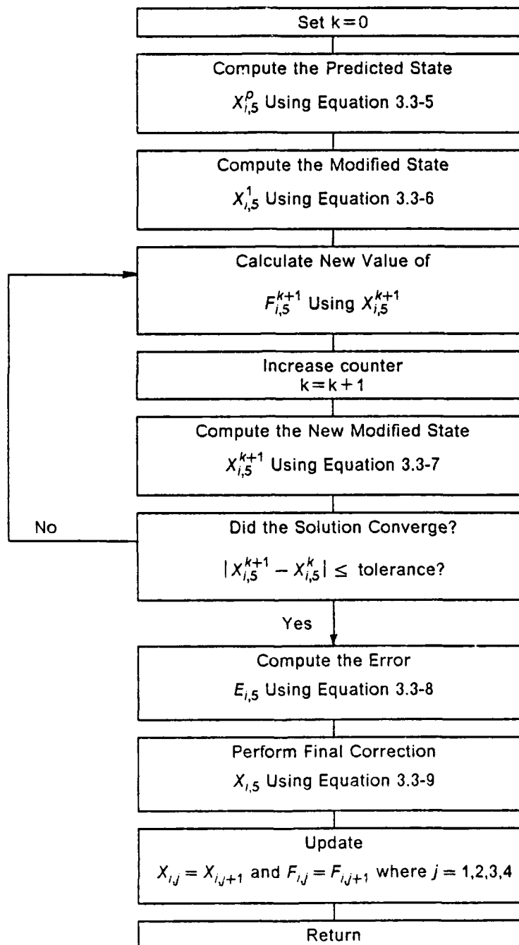
Figure 42. General Flow Chart of Predictor-Corrector Algorithm
