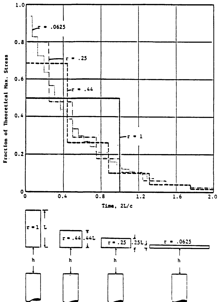
Figure 2-5 Effect of Impedance Ratio on the Theoretical Wave Shape for Same Hammer Mass and Drop. After Palacios (1977)
