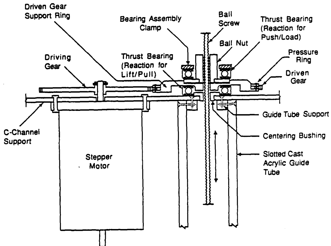
Figure 4-17 Ball Screw Assembly, Thrust Bearings, and Reaction Clamp
