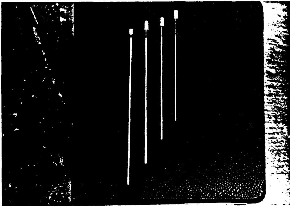
a) Individual Model Piles (Left to Right--49.3, 57.5, 69.8 and 86.0 g models)
