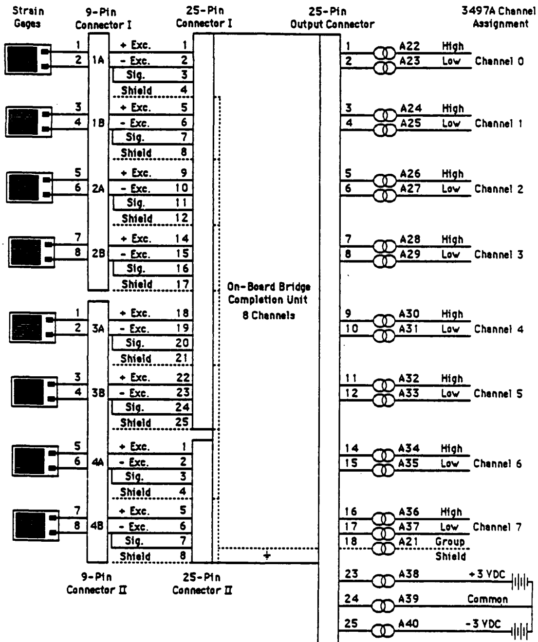
Figure 4-53 On-Board Bridge Completion Unit and Slip Ring Channel Assignments
