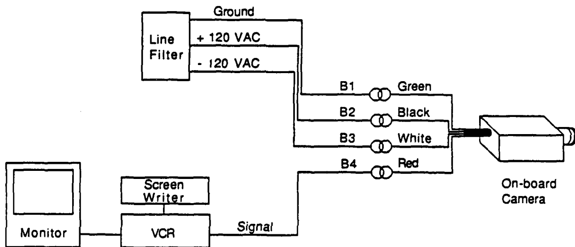
Figure 4-43 Closed Circuit Television Power Supply and Output Signal Circuit and Slip Ring Channel Assignments
