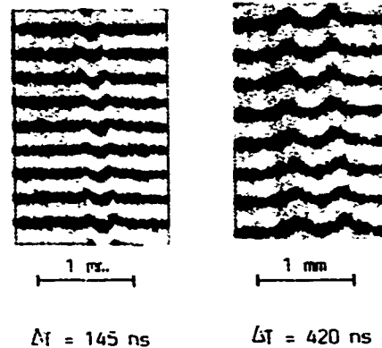
Figure 5 Discharge channel finite fringe interferograms
