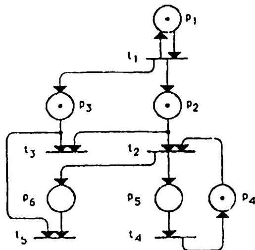
Figure B-23. Contention Between Transitions t_2 and t_3
