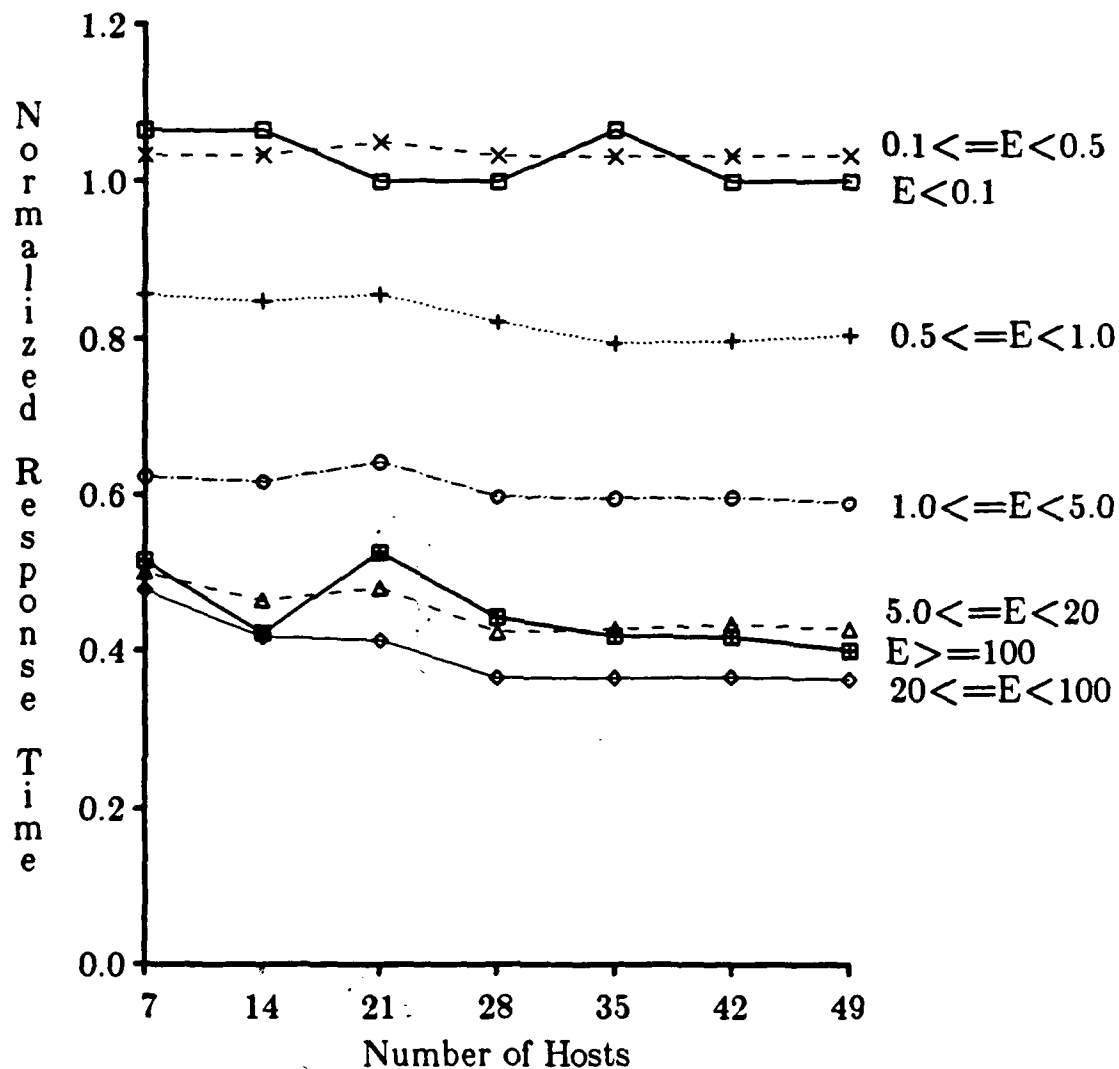
Figure 3.15. Average response times for several sizes of jobs (28 hosts; GLOBAL, T_i=1.0 , T_{CPU}=1.0s ; utilizations same as in Figure 3.2).
