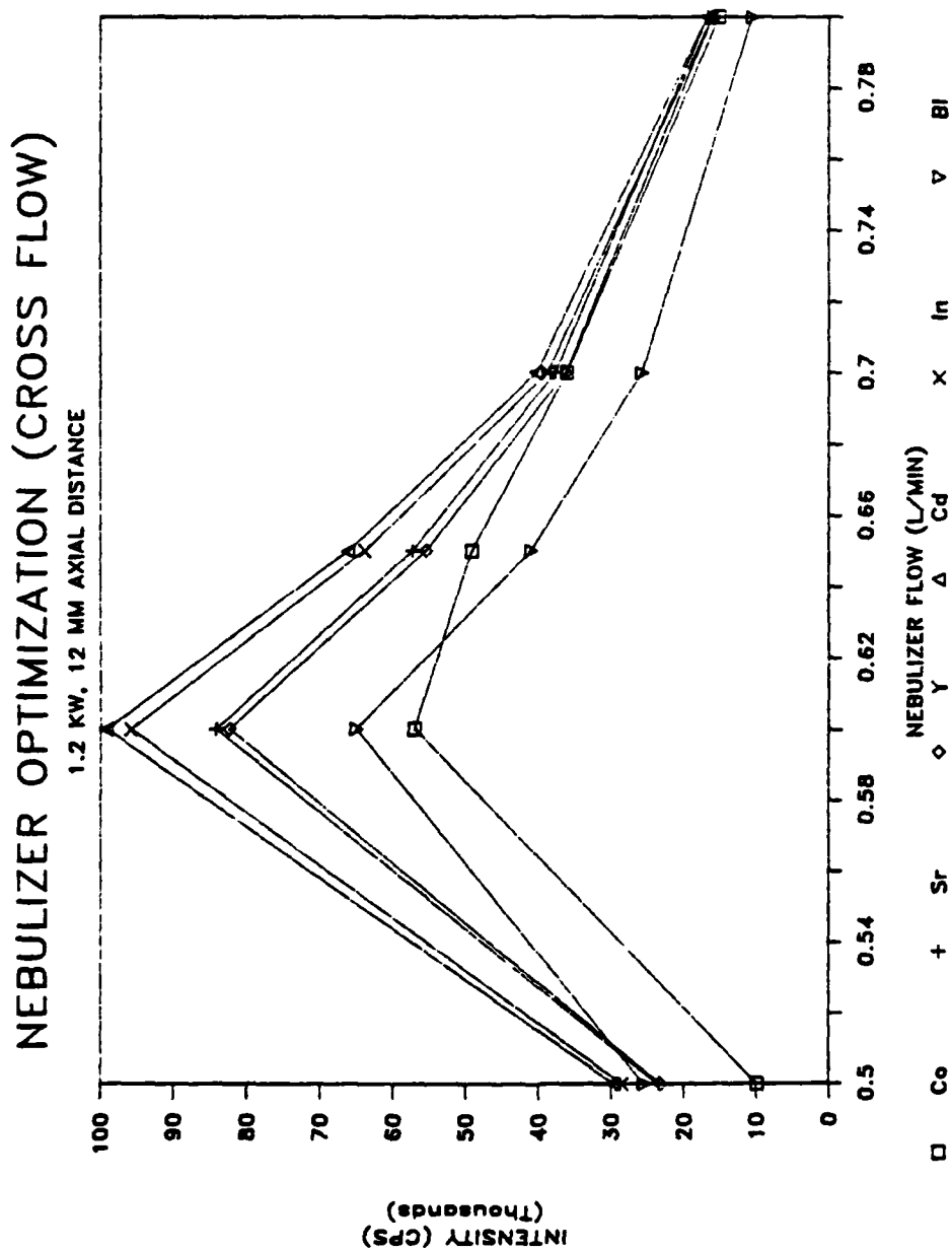
Figure 5-21. Nebulizer Flow vs. Signal Intensity @ 1.2 KW, 12 mm Sampling (cross flow)
