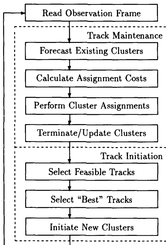
Figure 1.2: Temporal Clustering Process
