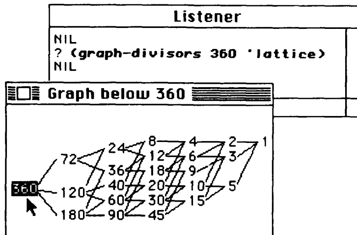
Figure 3: The integer divisors of 360.
