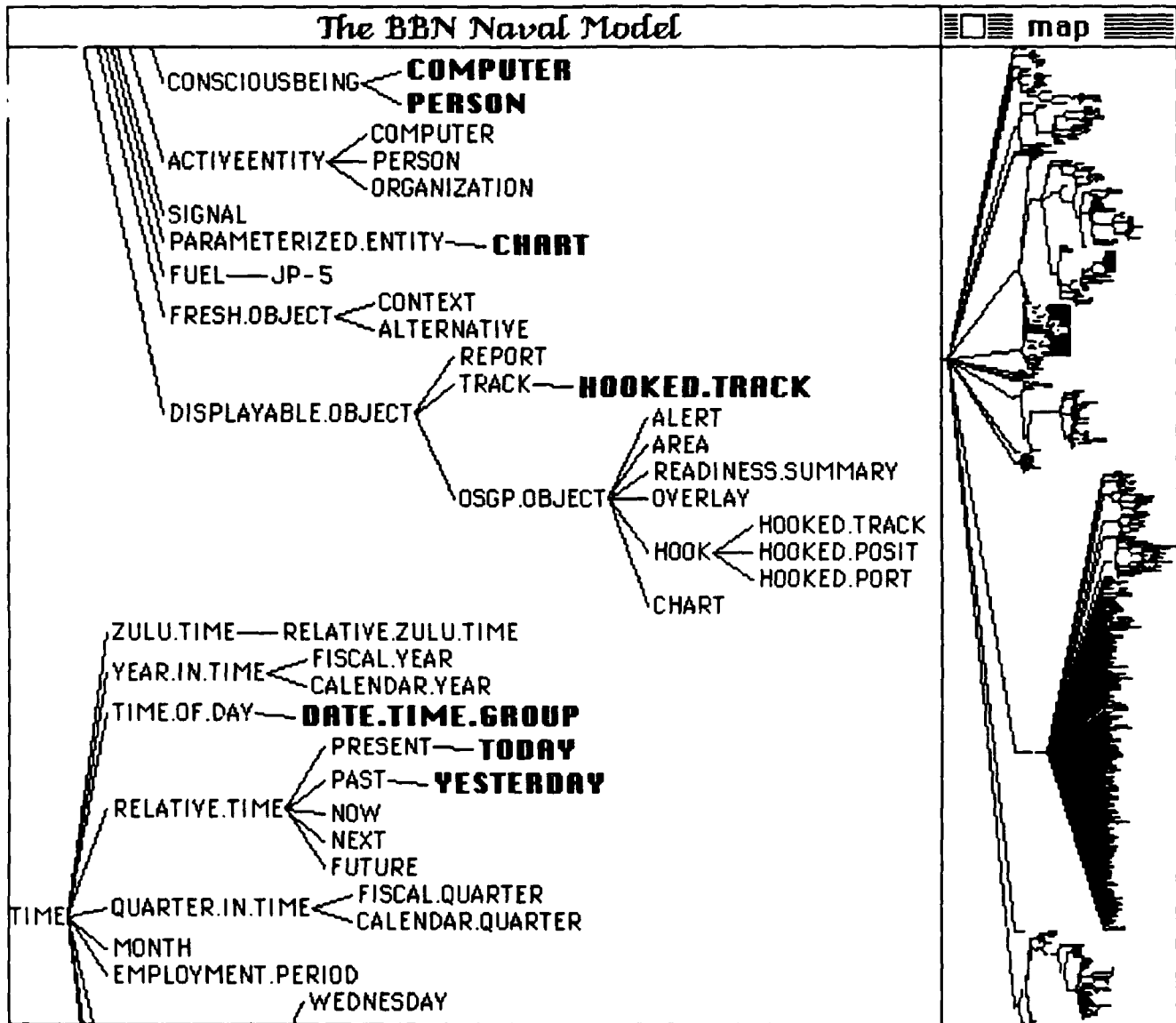
Figure 4: A typical medium-sized NIKL taxonomy.
