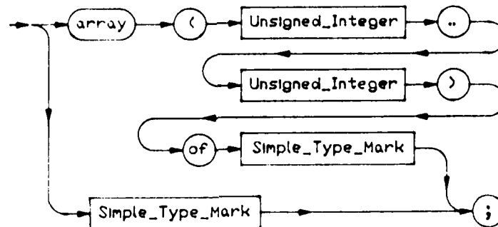
Figure 4. Syntax Diagram of Structure_Type
