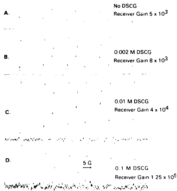
Fig. 3. ESR spectra following photolysis (313 nm) of solutions containing potassium ferrocyanide (0.1 M), DMPO (0.01 M) and varying concentrations of DSCG.
