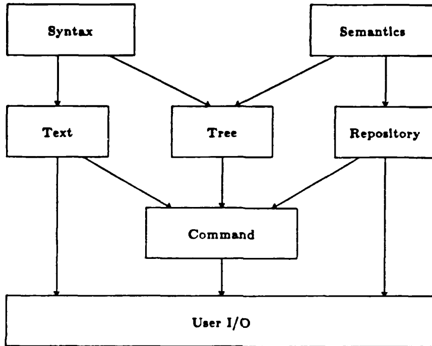
Figure 3: Component Dependencies in Pan
