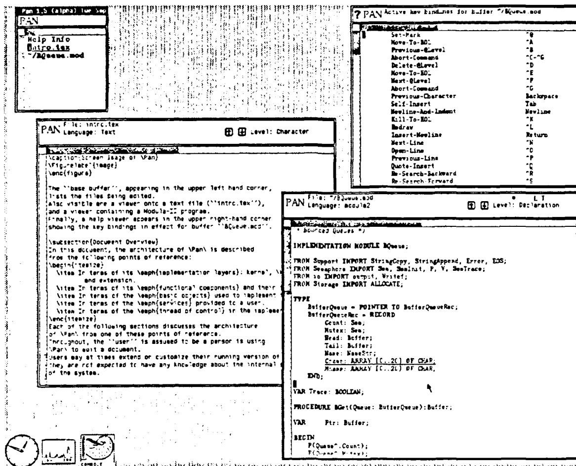
Figure 1: Screen Image of Pan
