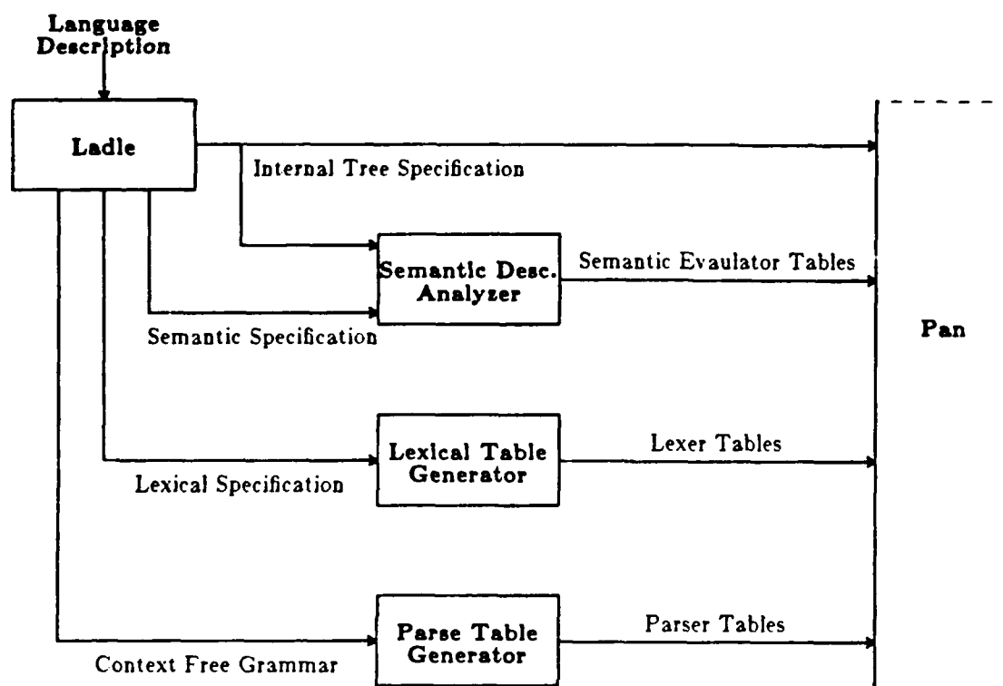
Figure 4: Flow of Information between Ladle and Pan
