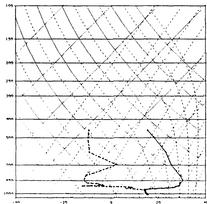
Fig. 36. Research Vessel POINT SUR Rawinsonde Soundings: 13 July 1987 1758 UTC (top) and 14 July 1987 1802 UTC (bottom), station location 33.5°N 120°W.
