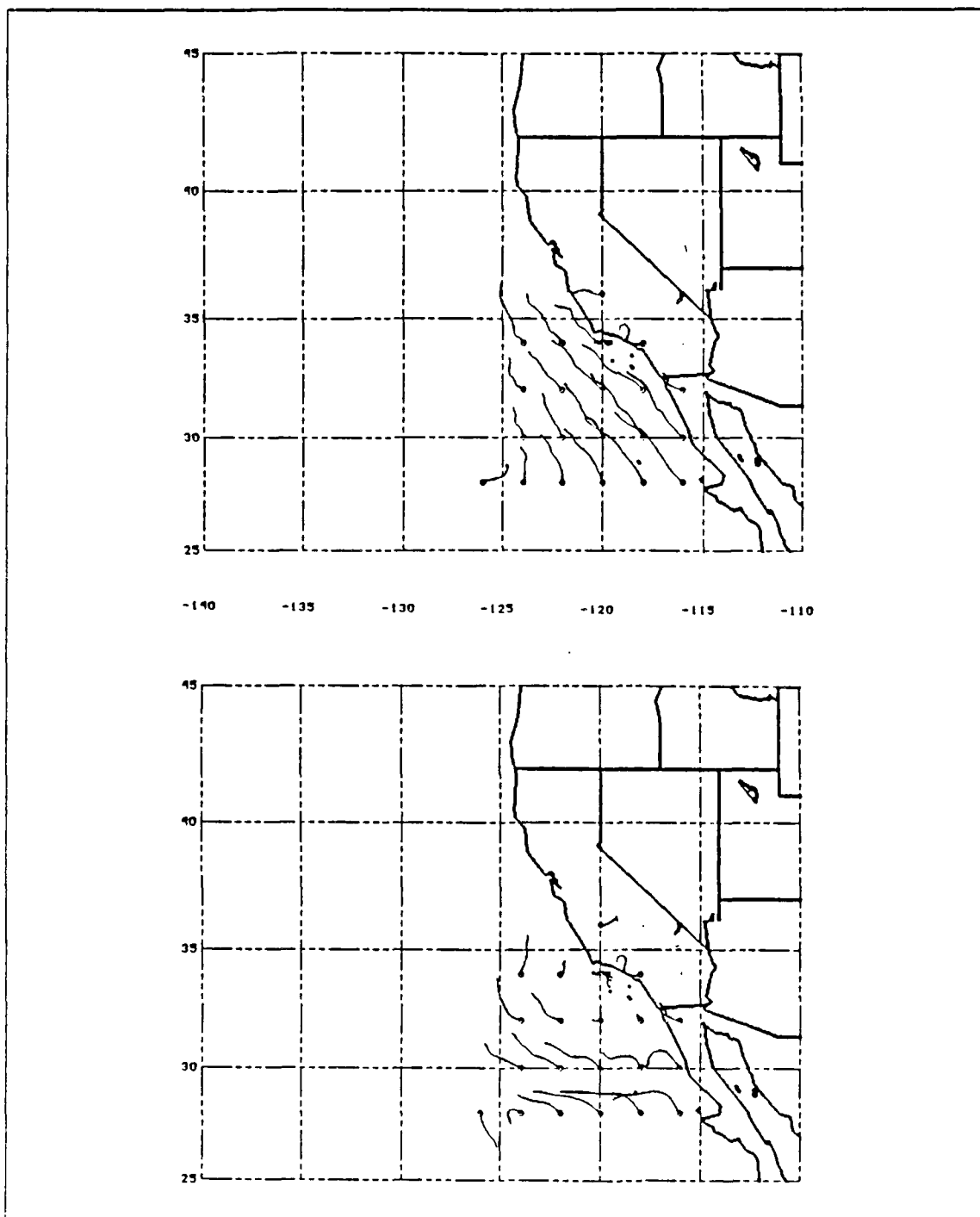
Fig. 39. NORAPS 13 July 1987 00-24 UTC Parcel Trajectories: 1000 mb pressure at 24 UTC (top) and 925 mb pressure at 24 UTC (bottom), circle indicates 24 UTC position.
