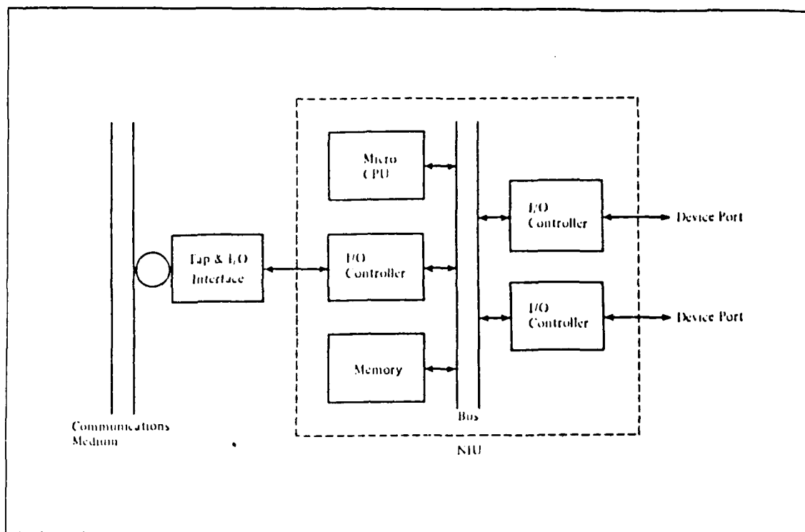
Figure 7. NIU Architecture
