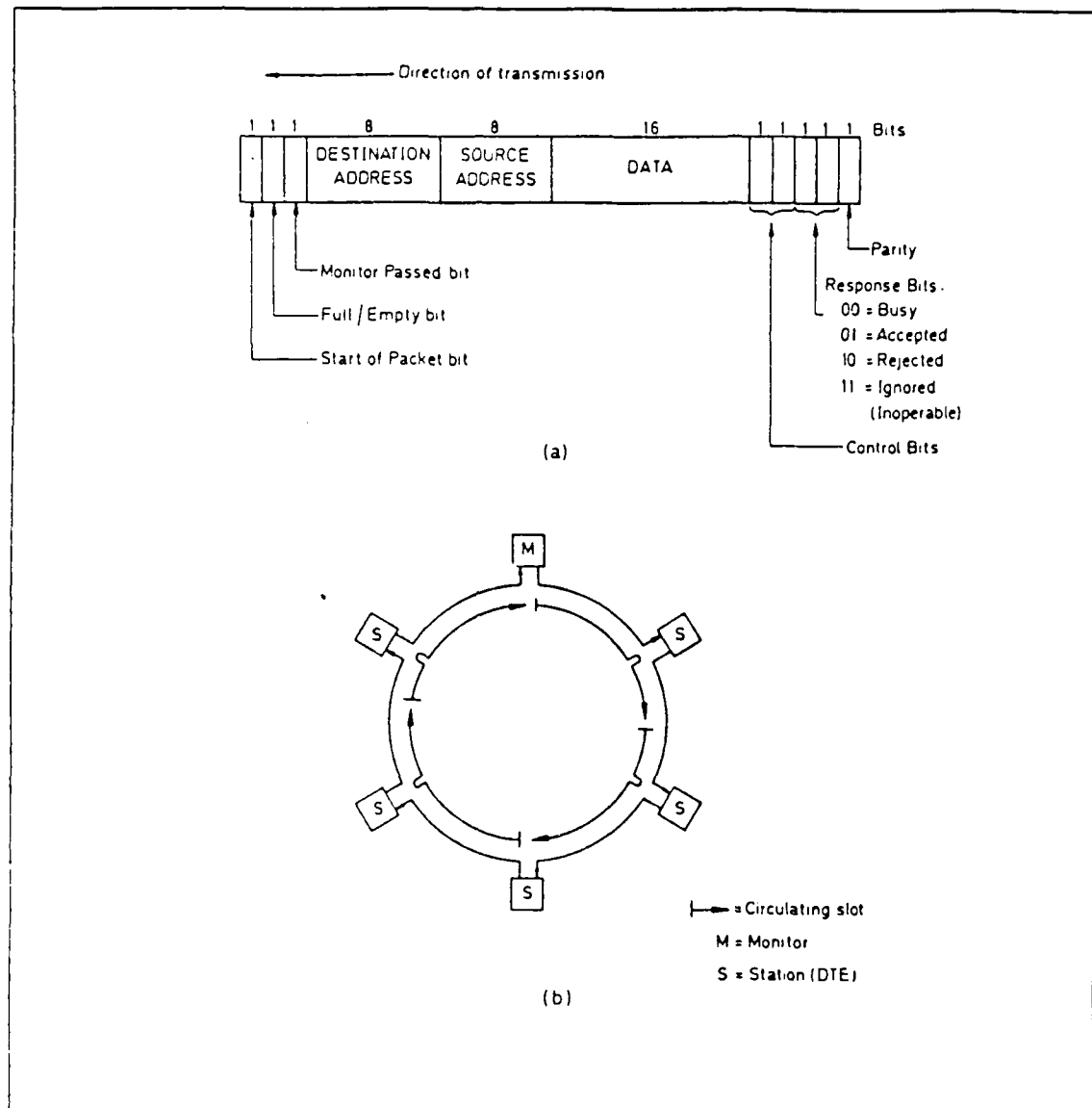
Figure 4. Slotted ring
