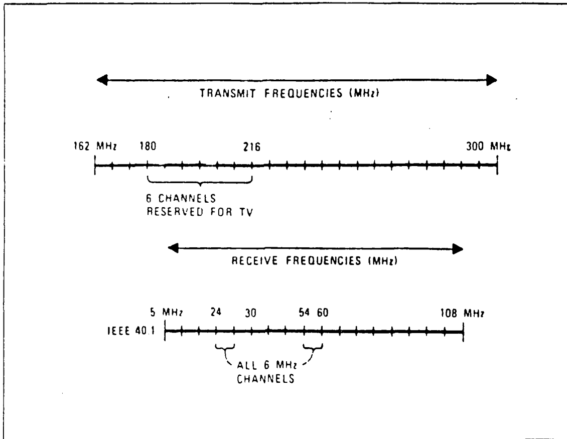
Figure 16. IEEE 40.1 Band Allocation
