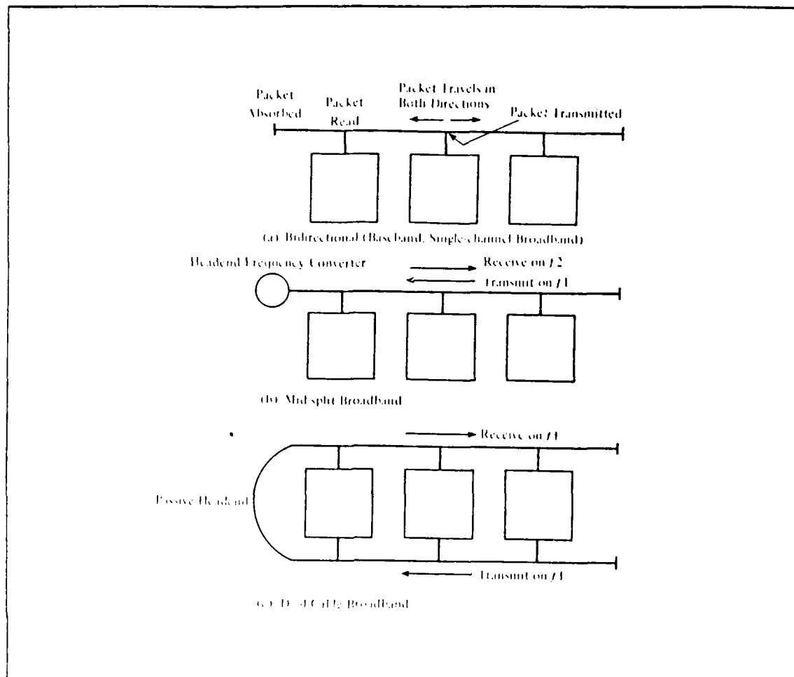
Figure 3. Transmission techniques
